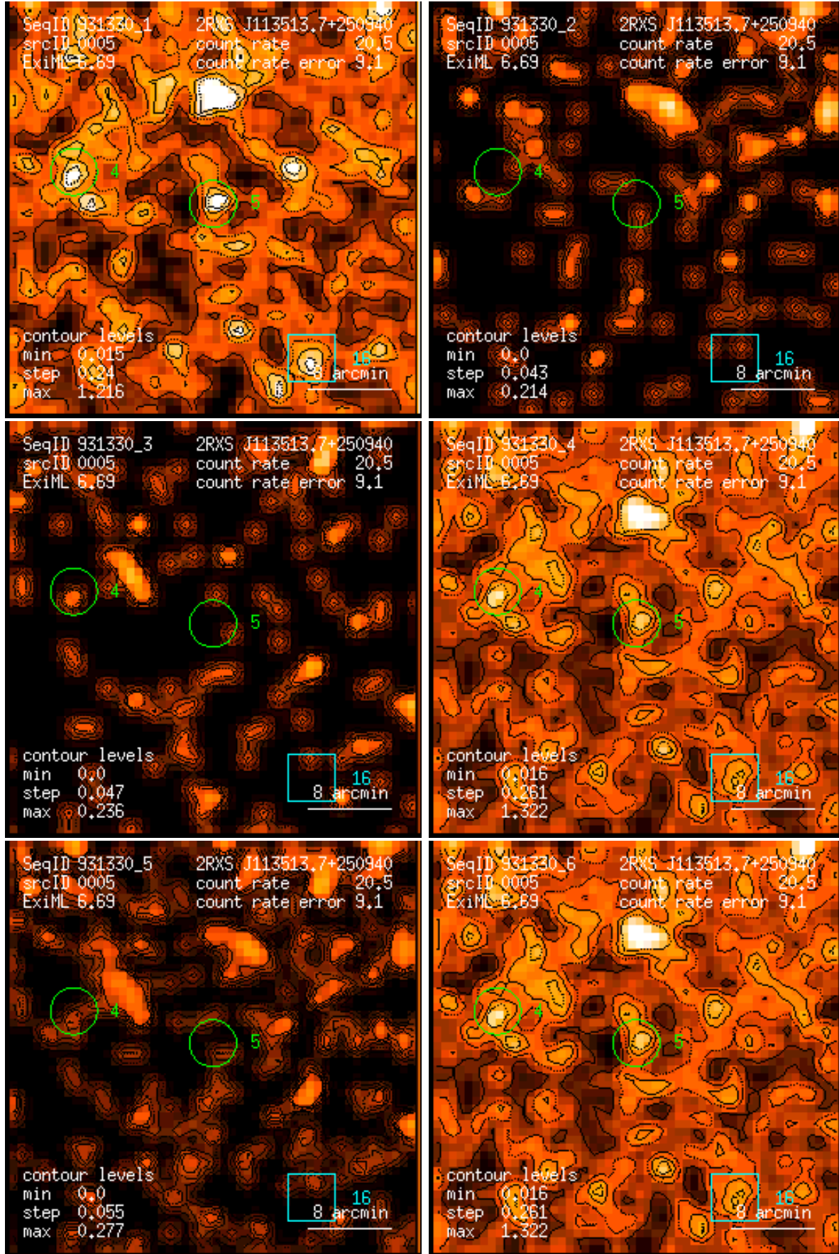
Figure 5: RASS 931330: detection 0005: band rate images, Gaussian filter: (1) PSPC channels 11 – 41, (2) 52 – 90, (3) 91 – 201, (4) 11 – 235, (5) 52 – 201, (6) 11 – 201. Broad band rates in counts/ks. Band rate contour levels in counts/ks/arcmin 2 .
