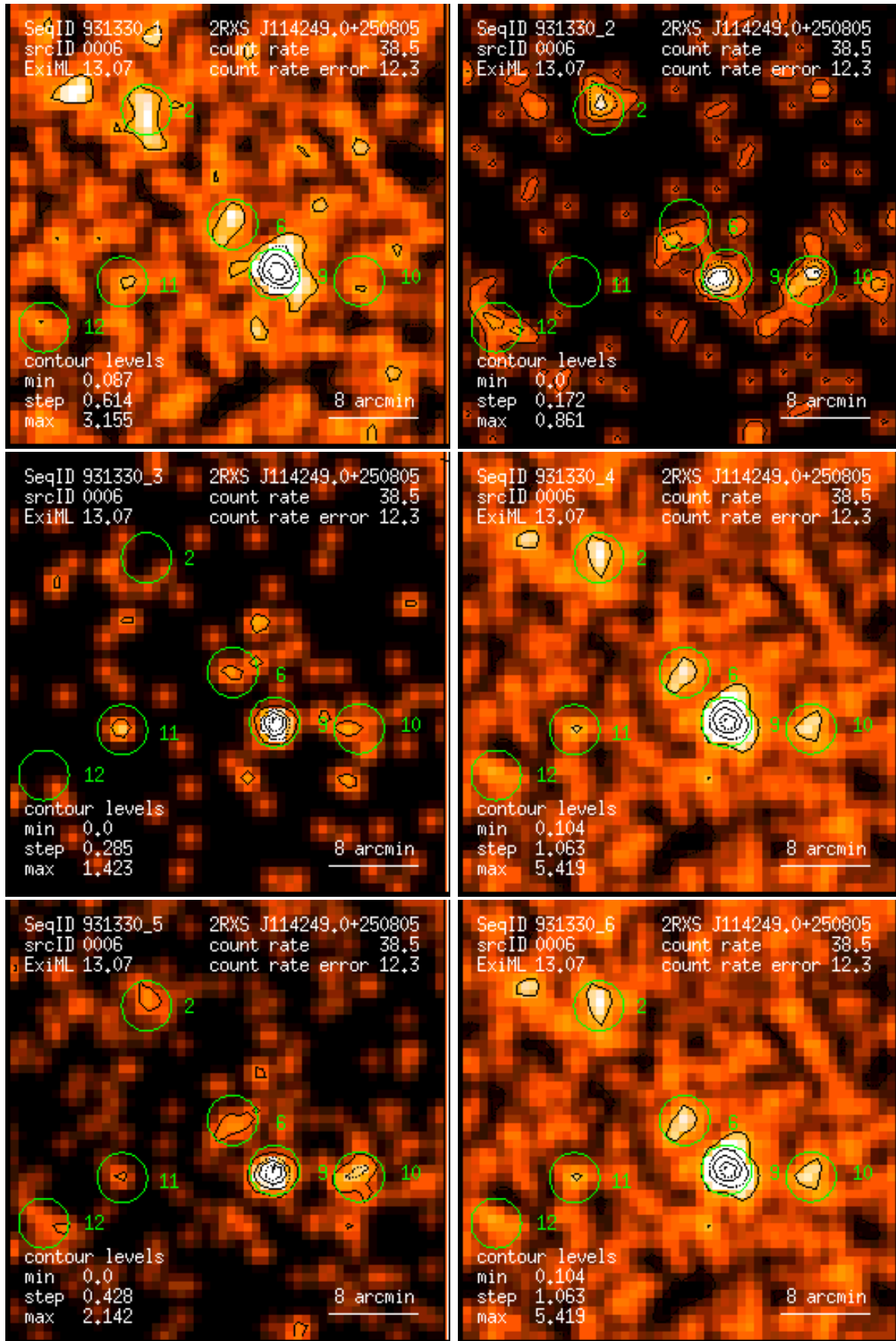
Figure 6: RASS 931330: detection 0006: band rate images, Gaussian filter: (1) PSPC channels 11 – 41, (2) 52 – 90, (3) 91 – 201, (4) 11 – 235, (5) 52 – 201, (6) 11 – 201. Broad band rates in counts/ks. Band rate contour levels in counts/ks/arcmin 2 .
