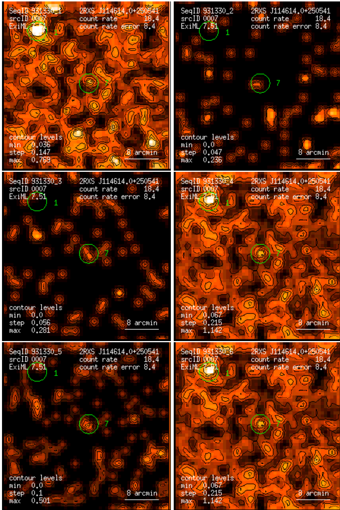
Figure 7: RASS 931330: detection 0007: band rate images, Gaussian filter: (1) PSPC channels 11 – 41, (2) 52 – 90, (3) 91 – 201, (4) 11 – 235, (5) 52 – 201, (6) 11 – 201. Broad band rates in counts/ks. Band rate contour levels in counts/ks/arcmin 2 .
