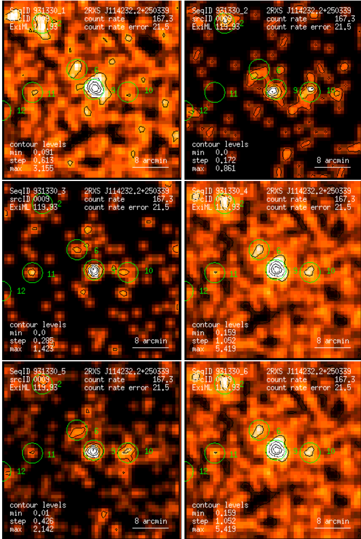
Figure 9: RASS 931330: detection 0009: band rate images, Gaussian filter: (1) PSPC channels 11 – 41, (2) 52 – 90, (3) 91 – 201, (4) 11 – 235, (5) 52 – 201, (6) 11 – 201. Broad band rates in counts/ks. Band rate contour levels in counts/ks/arcmin 2 .
