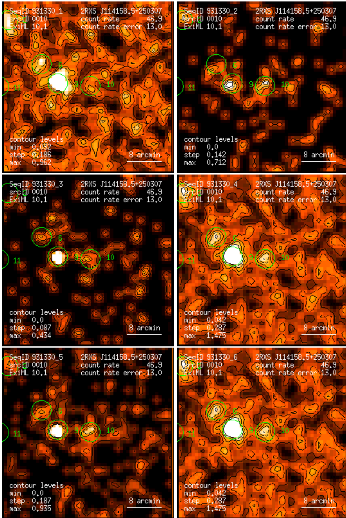
Figure 10: RASS 931330: detection 0010: band rate images, Gaussian filter: (1) PSPC channels 11 – 41, (2) 52 – 90, (3) 91 – 201, (4) 11 – 235, (5) 52 – 201, (6) 11 – 201. Broad band rates in counts/ks. Band rate contour levels in counts/ks/arcmin 2 .
