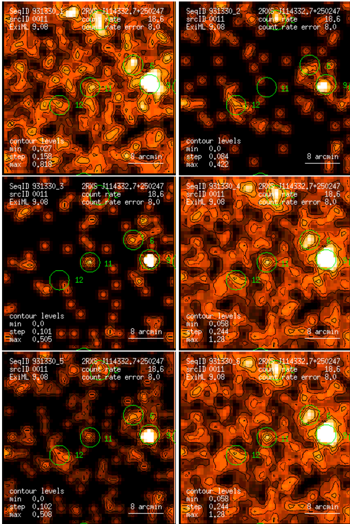
Figure 11: RASS 931330: detection 0011: band rate images, Gaussian filter: (1) PSPC channels 11 – 41, (2) 52 – 90, (3) 91 – 201, (4) 11 – 235, (5) 52 – 201, (6) 11 – 201. Broad band rates in counts/ks. Band rate contour levels in counts/ks/arcmin 2 .
