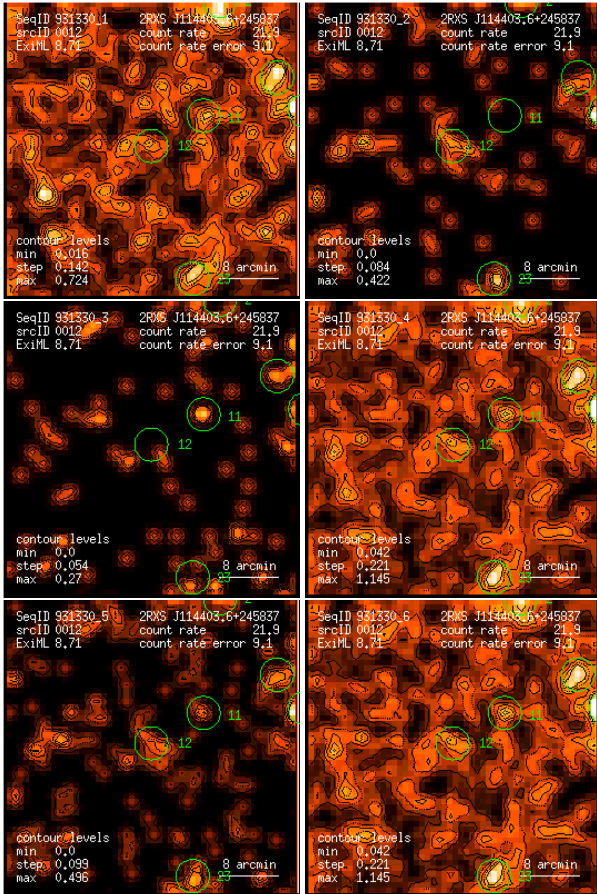
Figure 12: RASS 931330: detection 0012: band rate images, Gaussian filter: (1) PSPC channels 11 – 41, (2) 52 – 90, (3) 91 – 201, (4) 11 – 235, (5) 52 – 201, (6) 11 – 201. Broad band rates in counts/ks. Band rate contour levels in counts/ks/arcmin 2 .
