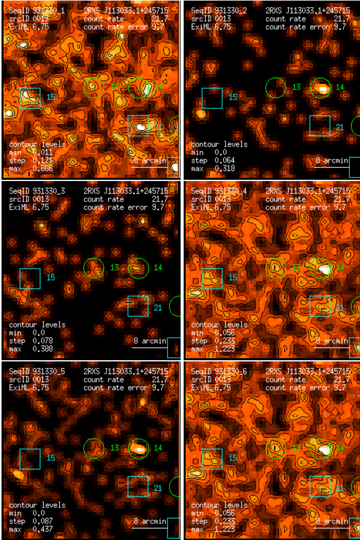
Figure 13: RASS 931330: detection 0013: band rate images, Gaussian filter: (1) PSPC channels 11 – 41, (2) 52 – 90, (3) 91 – 201, (4) 11 – 235, (5) 52 – 201, (6) 11 – 201. Broad band rates in counts/ks. Band rate contour levels in counts/ks/arcmin 2 .
