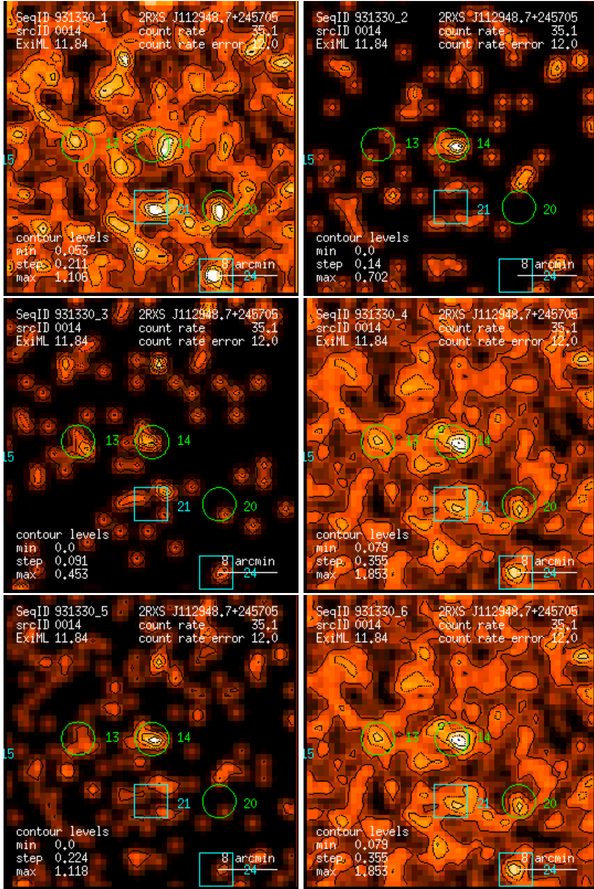
Figure 14: RASS 931330: detection 0014: band rate images, Gaussian filter: (1) PSPC channels 11 – 41, (2) 52 – 90, (3) 91 – 201, (4) 11 – 235, (5) 52 – 201, (6) 11 – 201. Broad band rates in counts/ks. Band rate contour levels in counts/ks/arcmin 2 .
