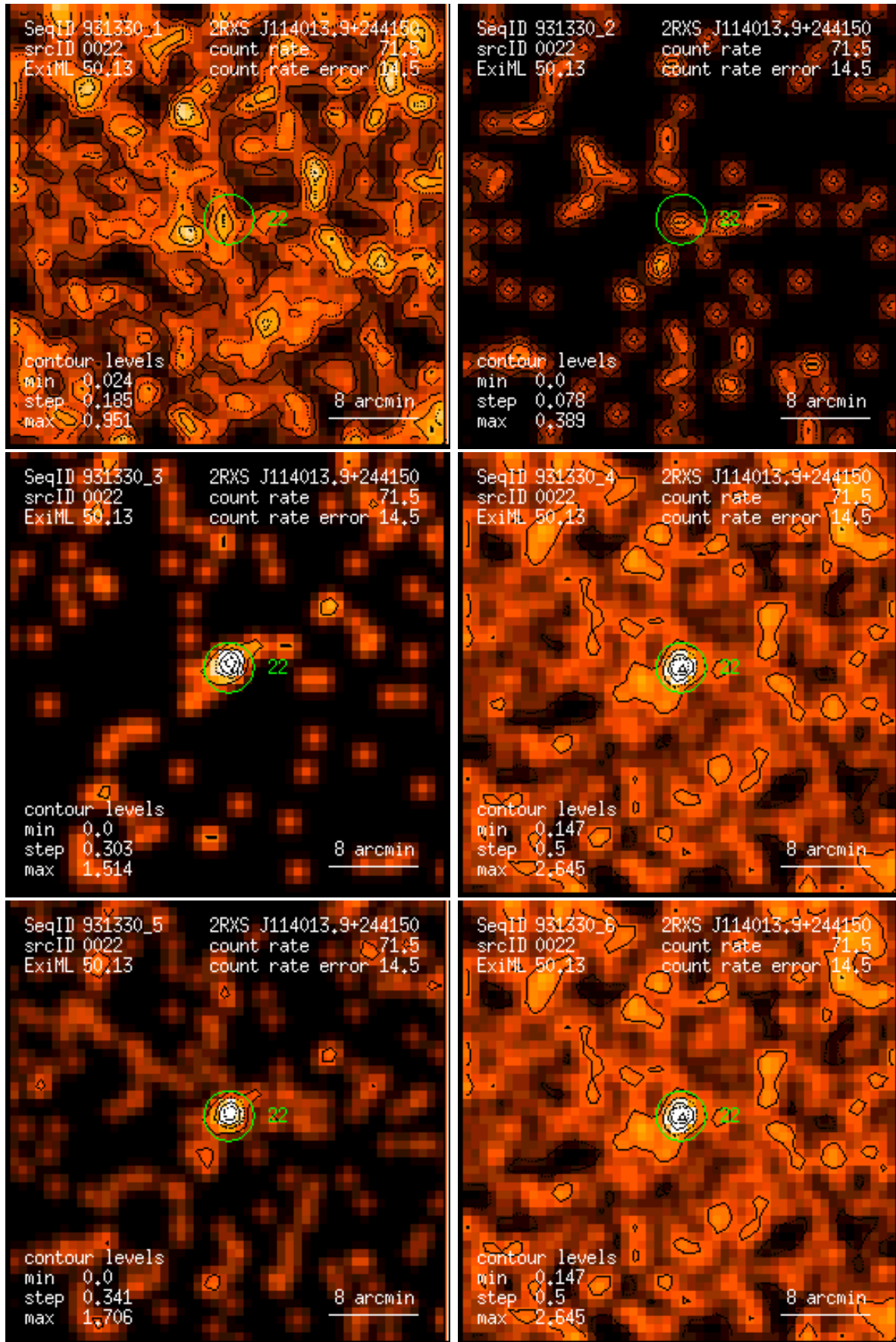
Figure 22: RASS 931330: detection 0022: band rate images, Gaussian filter: (1) PSPC channels 11 – 41, (2) 52 – 90, (3) 91 – 201, (4) 11 – 235, (5) 52 – 201, (6) 11 – 201. Broad band rates in counts/ks. Band rate contour levels in counts/ks/arcmin 2 .
