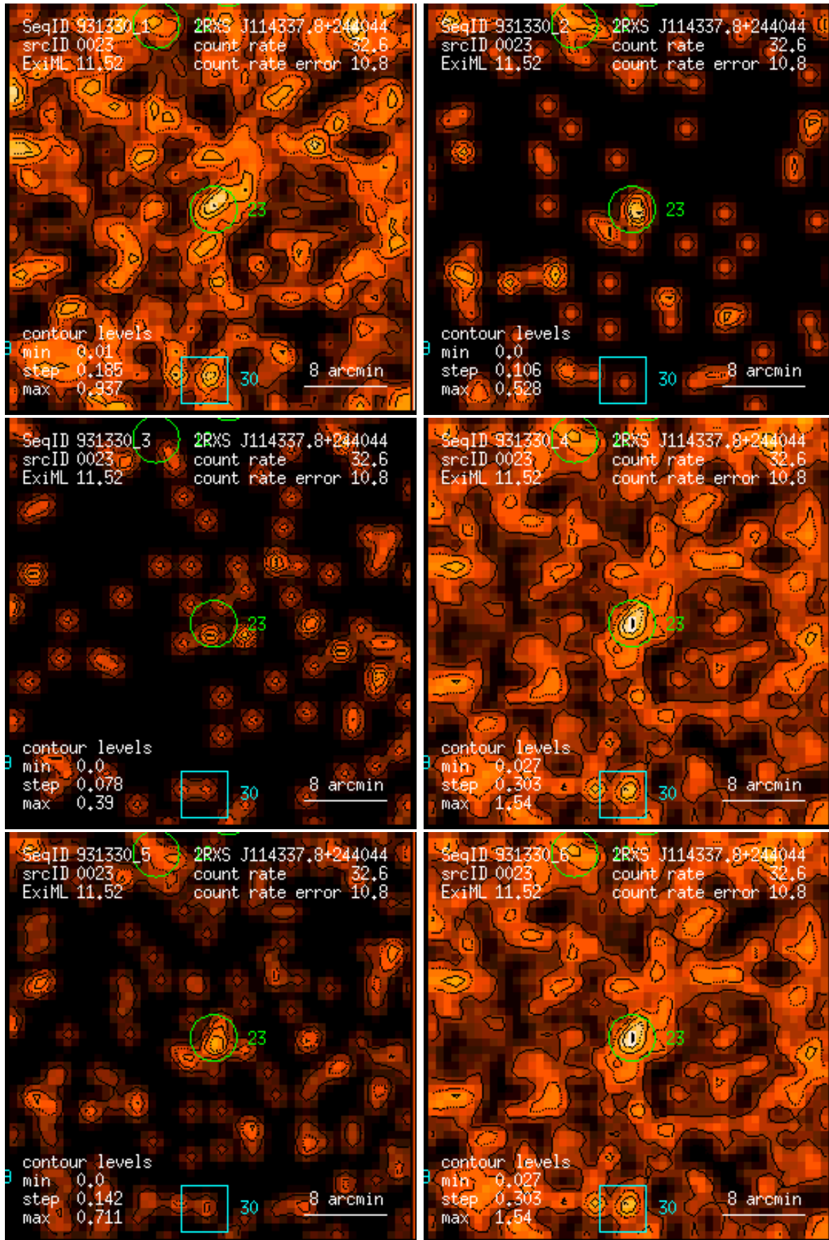
Figure 23: RASS 931330: detection 0023: band rate images, Gaussian filter: (1) PSPC channels 11 – 41, (2) 52 – 90, (3) 91 – 201, (4) 11 – 235, (5) 52 – 201, (6) 11 – 201. Broad band rates in counts/ks. Band rate contour levels in counts/ks/arcmin 2 .
