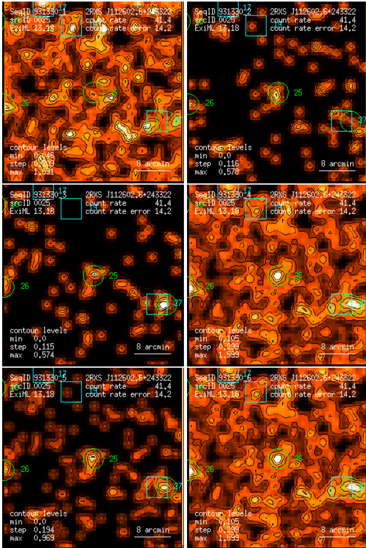
Figure 25: RASS 931330: detection 0025: band rate images, Gaussian filter: (1) PSPC channels 11 – 41, (2) 52 – 90, (3) 91 – 201, (4) 11 – 235, (5) 52 – 201, (6) 11 – 201. Broad band rates in counts/ks. Band rate contour levels in counts/ks/arcmin 2 .
