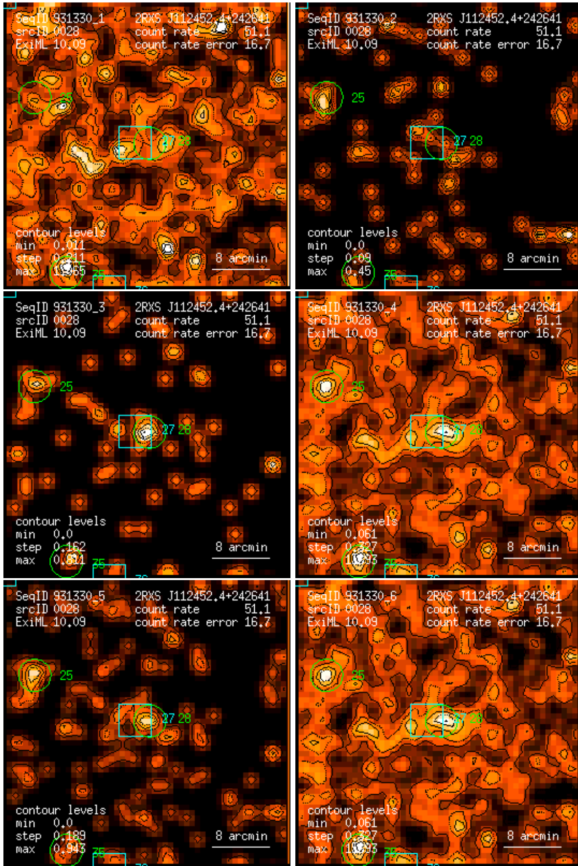
Figure 28: RASS 931330: detection 0028: band rate images, Gaussian filter: (1) PSPC channels 11 – 41, (2) 52 – 90, (3) 91 – 201, (4) 11 – 235, (5) 52 – 201, (6) 11 – 201. Broad band rates in counts/ks. Band rate contour levels in counts/ks/arcmin 2 .
