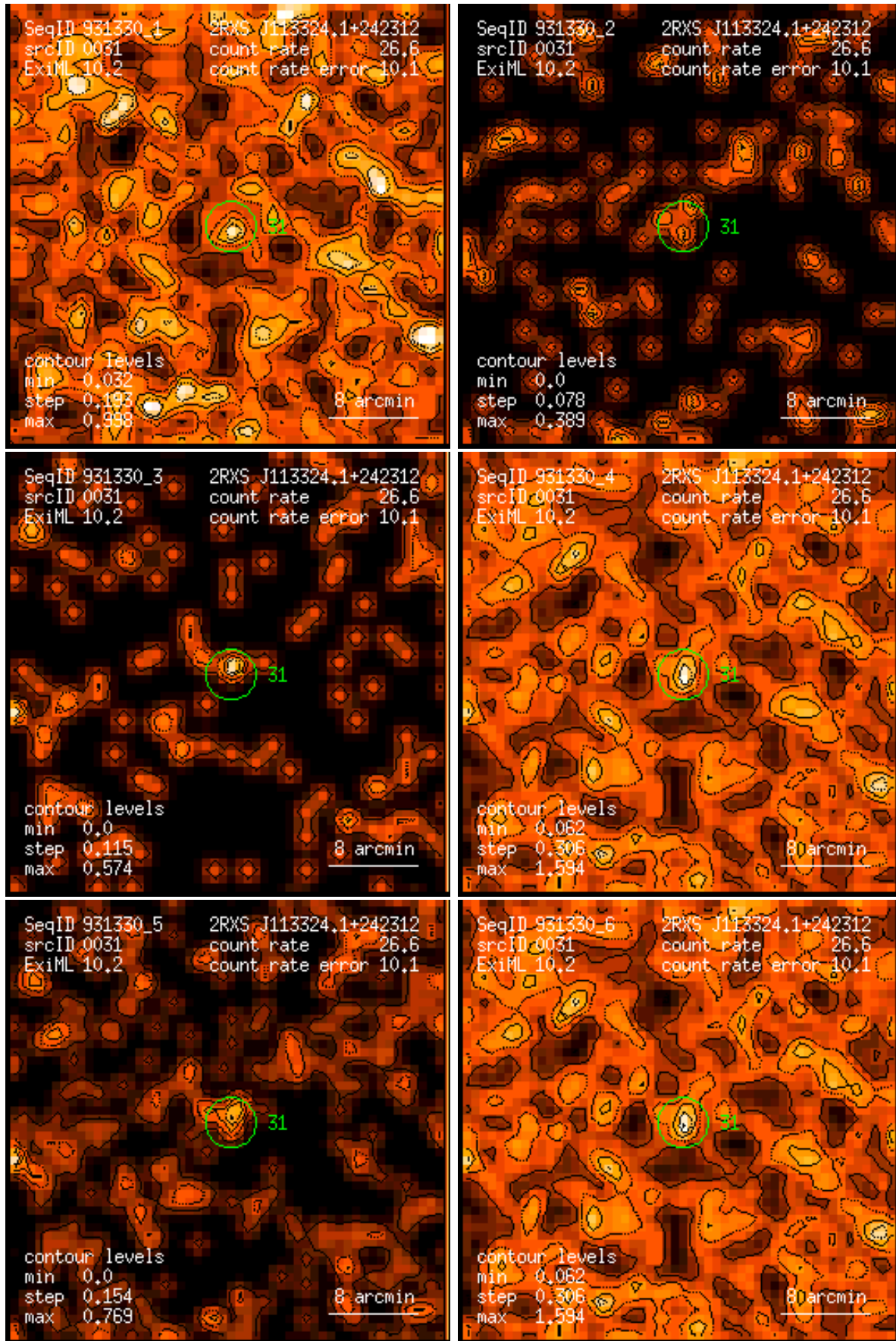
Figure 31: RASS 931330: detection 0031: band rate images, Gaussian filter: (1) PSPC channels 11 – 41, (2) 52 – 90, (3) 91 – 201, (4) 11 – 235, (5) 52 – 201, (6) 11 – 201. Broad band rates in counts/ks. Band rate contour levels in counts/ks/arcmin 2 .
