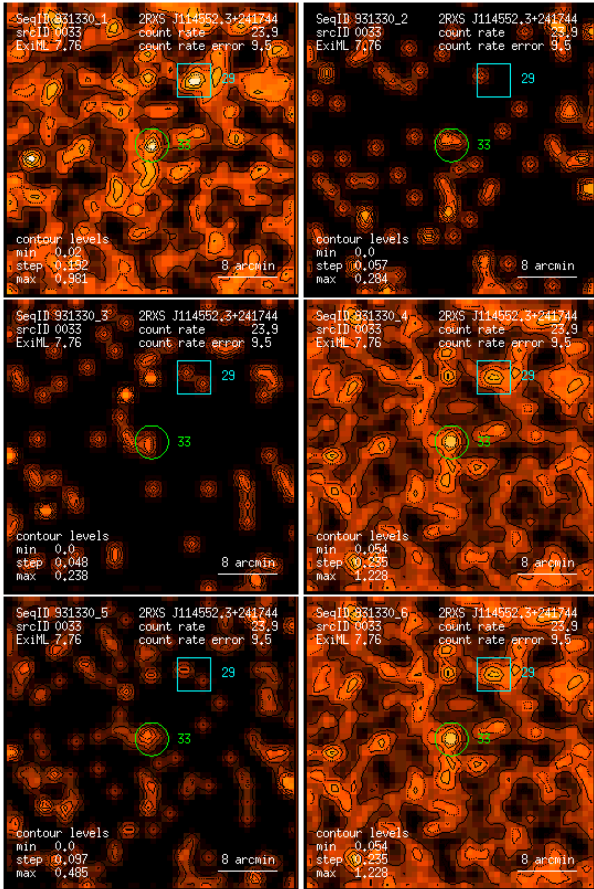
Figure 33: RASS 931330: detection 0033: band rate images, Gaussian filter: (1) PSPC channels 11 – 41, (2) 52 – 90, (3) 91 – 201, (4) 11 – 235, (5) 52 – 201, (6) 11 – 201. Broad band rates in counts/ks. Band rate contour levels in counts/ks/arcmin 2 .
