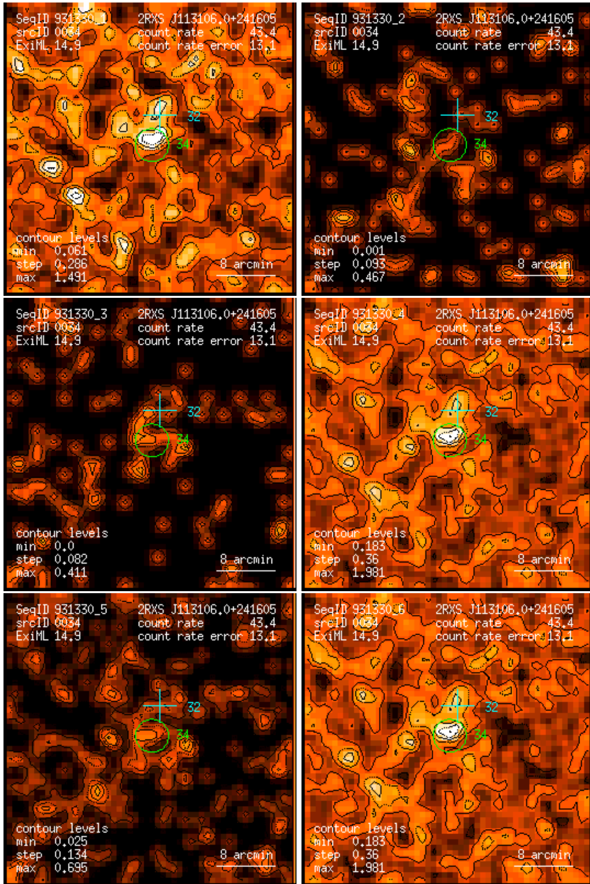
Figure 34: RASS 931330: detection 0034: band rate images, Gaussian filter: (1) PSPC channels 11 – 41, (2) 52 – 90, (3) 91 – 201, (4) 11 – 235, (5) 52 – 201, (6) 11 – 201. Broad band rates in counts/ks. Band rate contour levels in counts/ks/arcmin 2 .
