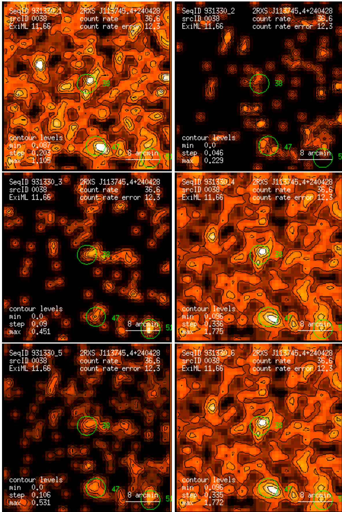
Figure 38: RASS 931330: detection 0038: band rate images, Gaussian filter: (1) PSPC channels 11 – 41, (2) 52 – 90, (3) 91 – 201, (4) 11 – 235, (5) 52 – 201, (6) 11 – 201. Broad band rates in counts/ks. Band rate contour levels in counts/ks/arcmin 2 .
