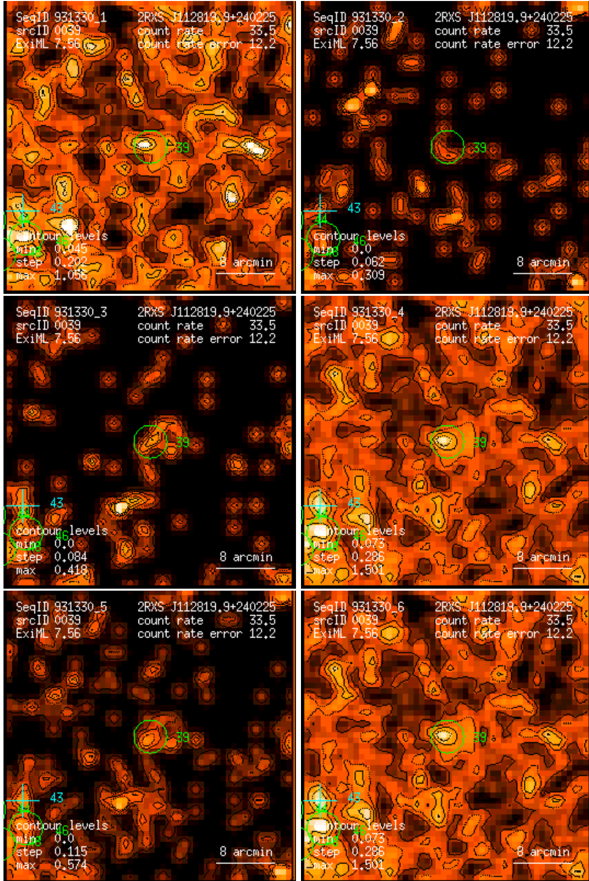
Figure 39: RASS 931330: detection 0039: band rate images, Gaussian filter: (1) PSPC channels 11 – 41, (2) 52 – 90, (3) 91 – 201, (4) 11 – 235, (5) 52 – 201, (6) 11 – 201. Broad band rates in counts/ks. Band rate contour levels in counts/ks/arcmin 2 .
