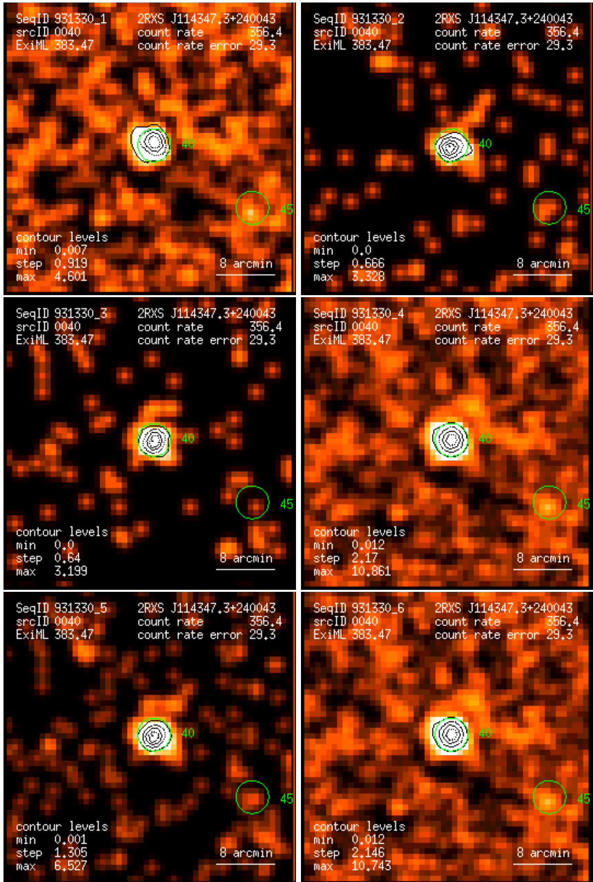
Figure 40: RASS 931330: detection 0040: band rate images, Gaussian filter: (1) PSPC channels 11 – 41, (2) 52 – 90, (3) 91 – 201, (4) 11 – 235, (5) 52 – 201, (6) 11 – 201. Broad band rates in counts/ks. Band rate contour levels in counts/ks/arcmin 2 .
