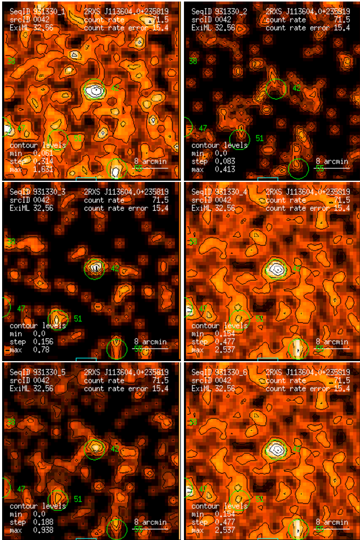
Figure 42: RASS 931330: detection 0042: band rate images, Gaussian filter: (1) PSPC channels 11 – 41, (2) 52 – 90, (3) 91 – 201, (4) 11 – 235, (5) 52 – 201, (6) 11 – 201. Broad band rates in counts/ks. Band rate contour levels in counts/ks/arcmin 2 .
