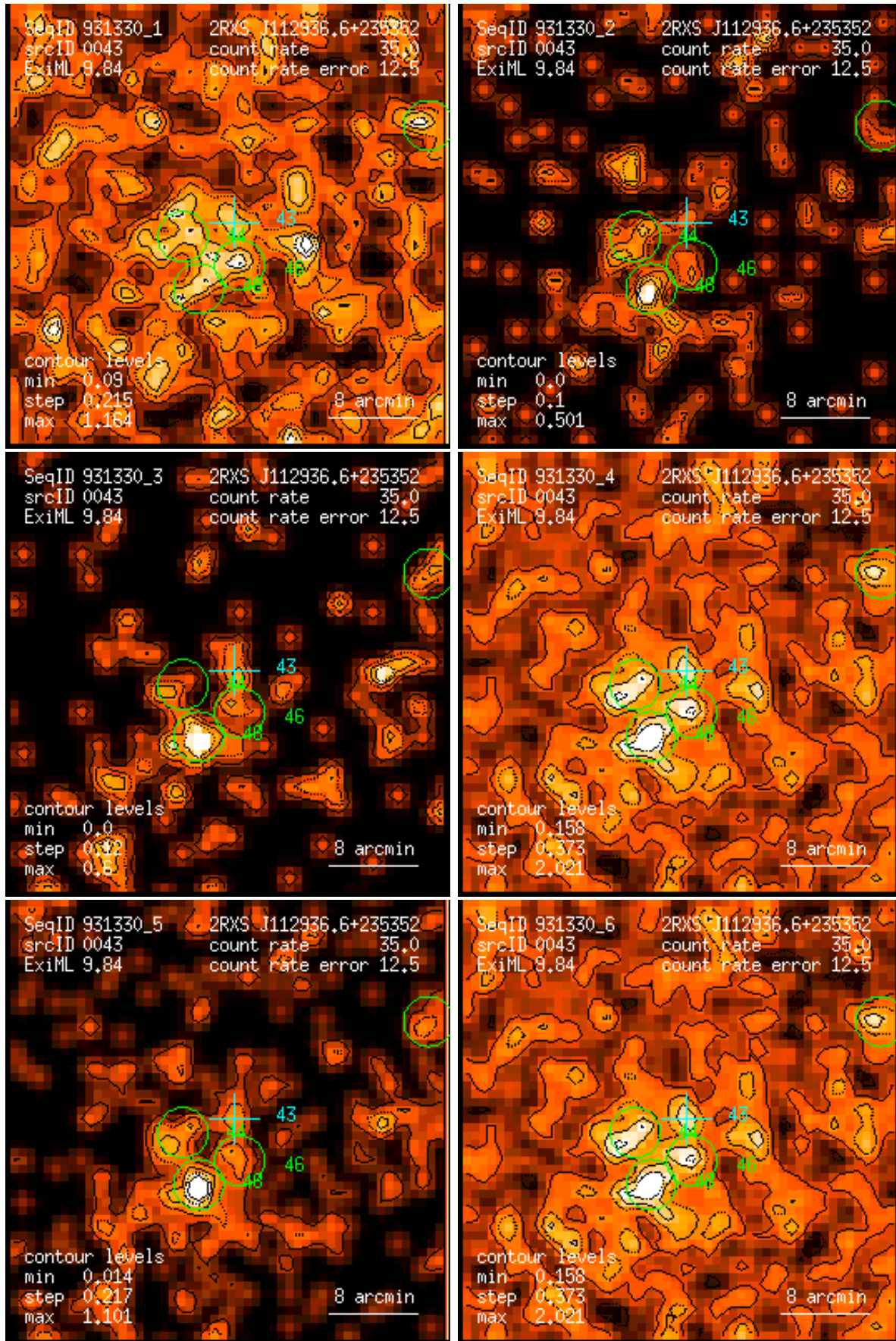
Figure 43: RASS 931330: detection 0043: band rate images, Gaussian filter: (1) PSPC channels 11 – 41, (2) 52 – 90, (3) 91 – 201, (4) 11 – 235, (5) 52 – 201, (6) 11 – 201. Broad band rates in counts/ks. Band rate contour levels in counts/ks/arcmin 2 .
