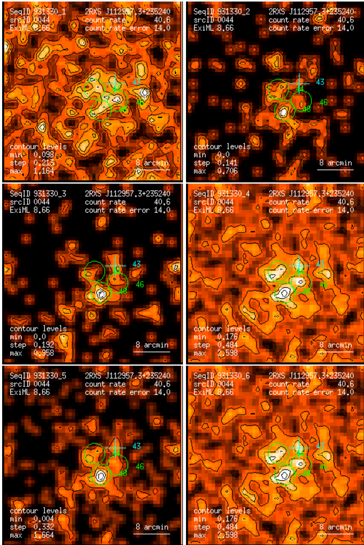
Figure 44: RASS 931330: detection 0044: band rate images, Gaussian filter: (1) PSPC channels 11 – 41, (2) 52 – 90, (3) 91 – 201, (4) 11 – 235, (5) 52 – 201, (6) 11 – 201. Broad band rates in counts/ks. Band rate contour levels in counts/ks/arcmin 2 .
