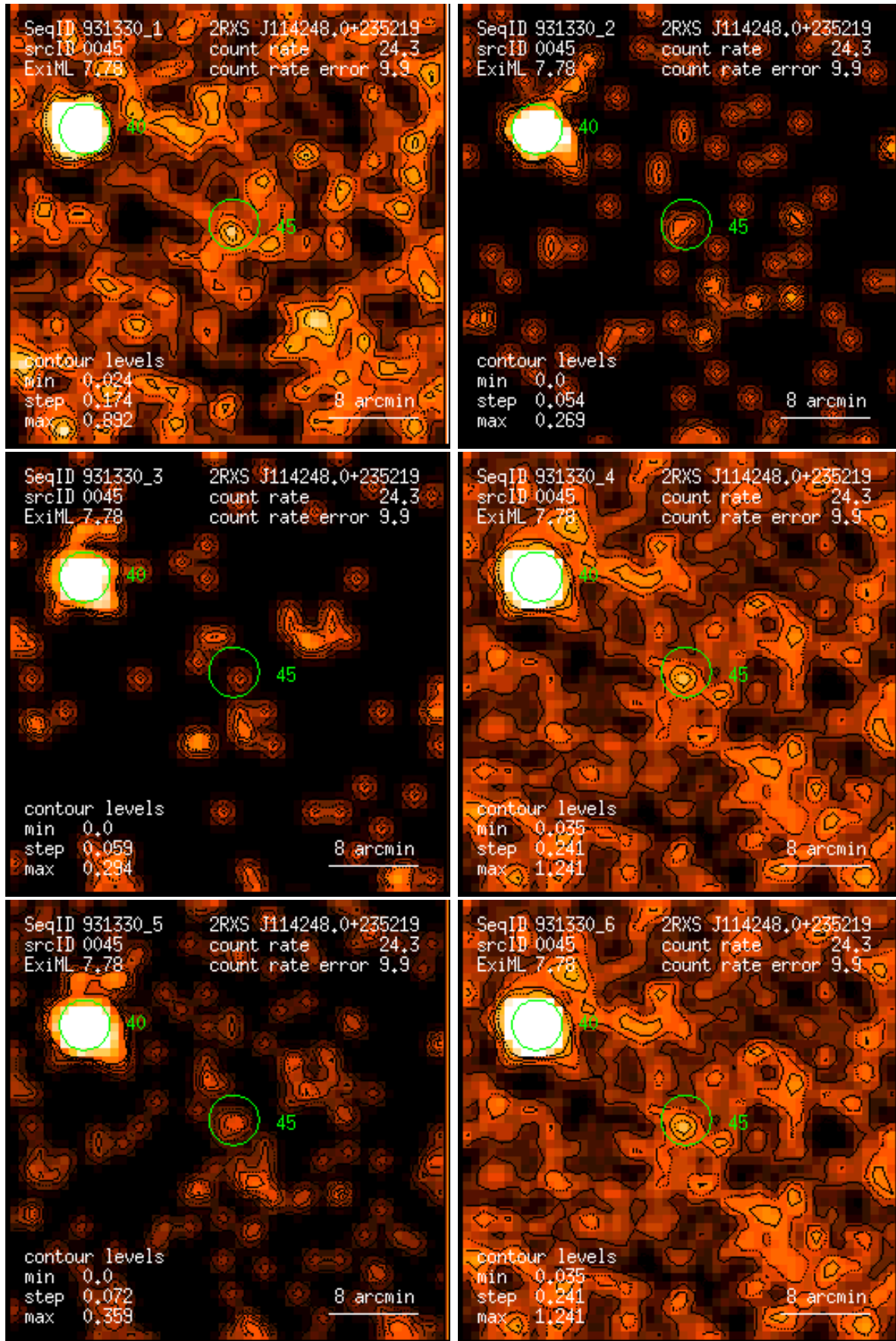
Figure 45: RASS 931330: detection 0045: band rate images, Gaussian filter: (1) PSPC channels 11 – 41, (2) 52 – 90, (3) 91 – 201, (4) 11 – 235, (5) 52 – 201, (6) 11 – 201. Broad band rates in counts/ks. Band rate contour levels in counts/ks/arcmin 2 .
