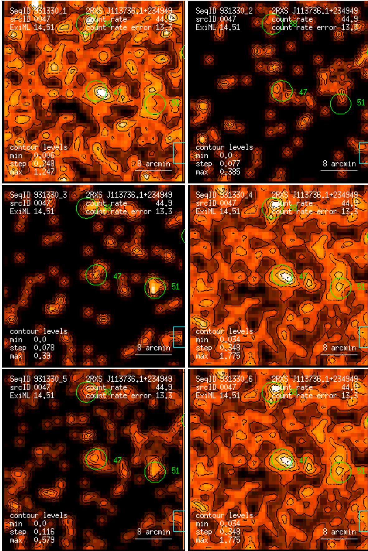
Figure 47: RASS 931330: detection 0047: band rate images, Gaussian filter: (1) PSPC channels 11 – 41, (2) 52 – 90, (3) 91 – 201, (4) 11 – 235, (5) 52 – 201, (6) 11 – 201. Broad band rates in counts/ks. Band rate contour levels in counts/ks/arcmin 2 .
