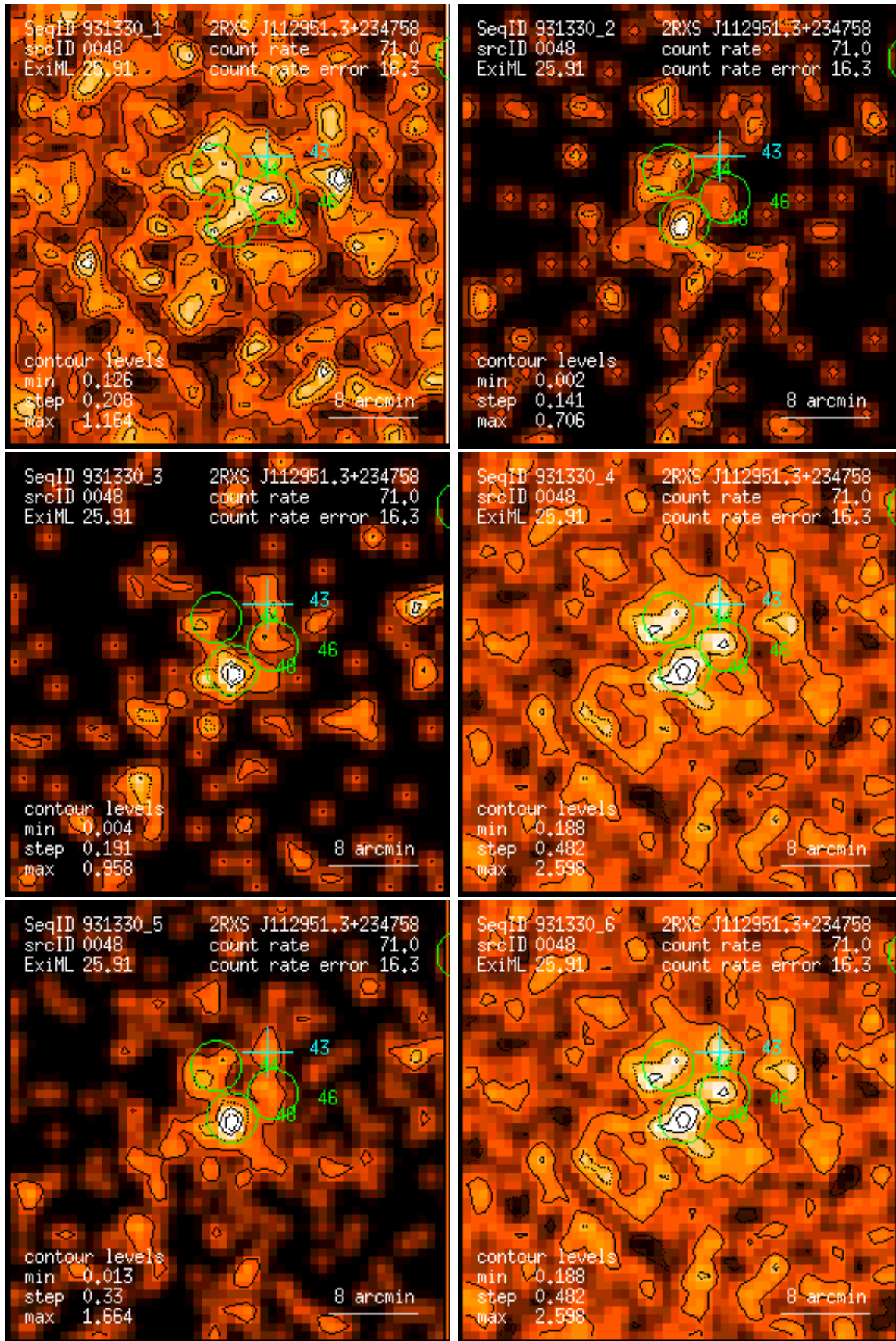
Figure 48: RASS 931330: detection 0048: band rate images, Gaussian filter: (1) PSPC channels 11 – 41, (2) 52 – 90, (3) 91 – 201, (4) 11 – 235, (5) 52 – 201, (6) 11 – 201. Broad band rates in counts/ks. Band rate contour levels in counts/ks/arcmin 2 .
