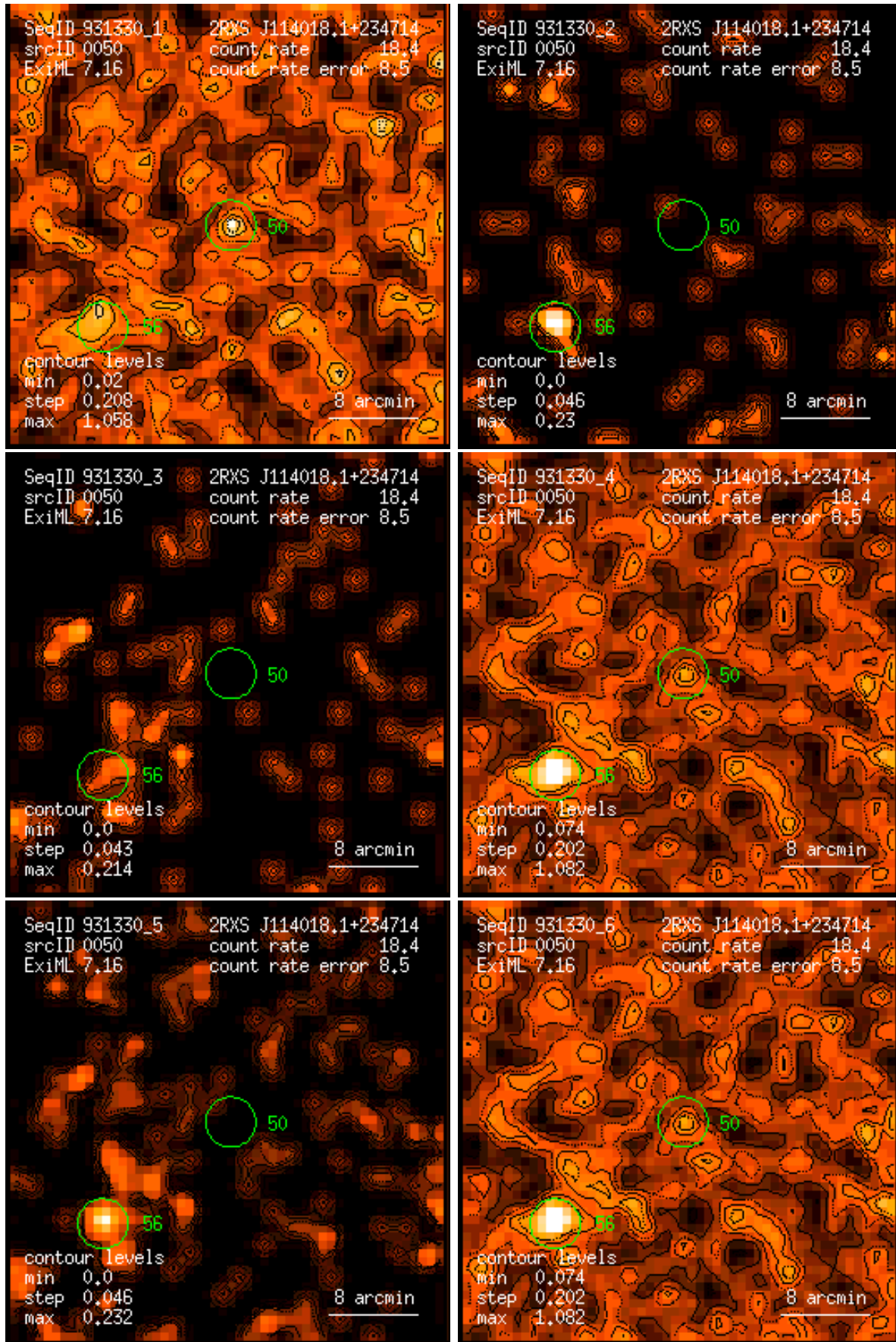
Figure 50: RASS 931330: detection 0050: band rate images, Gaussian filter: (1) PSPC channels 11 – 41, (2) 52 – 90, (3) 91 – 201, (4) 11 – 235, (5) 52 – 201, (6) 11 – 201. Broad band rates in counts/ks. Band rate contour levels in counts/ks/arcmin 2 .
