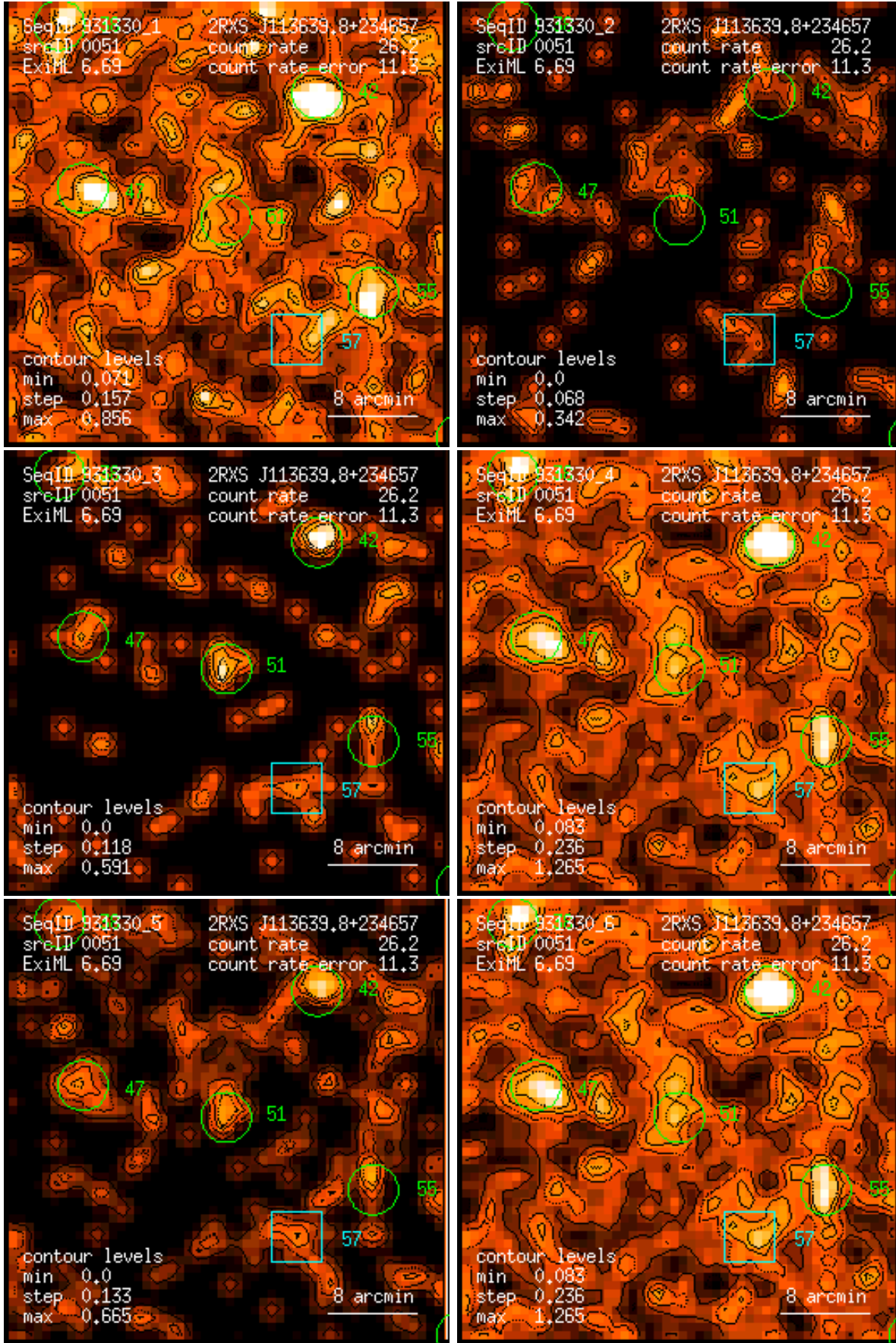
Figure 51: RASS 931330: detection 0051: band rate images, Gaussian filter: (1) PSPC channels 11 – 41, (2) 52 – 90, (3) 91 – 201, (4) 11 – 235, (5) 52 – 201, (6) 11 – 201. Broad band rates in counts/ks. Band rate contour levels in counts/ks/arcmin 2 .
