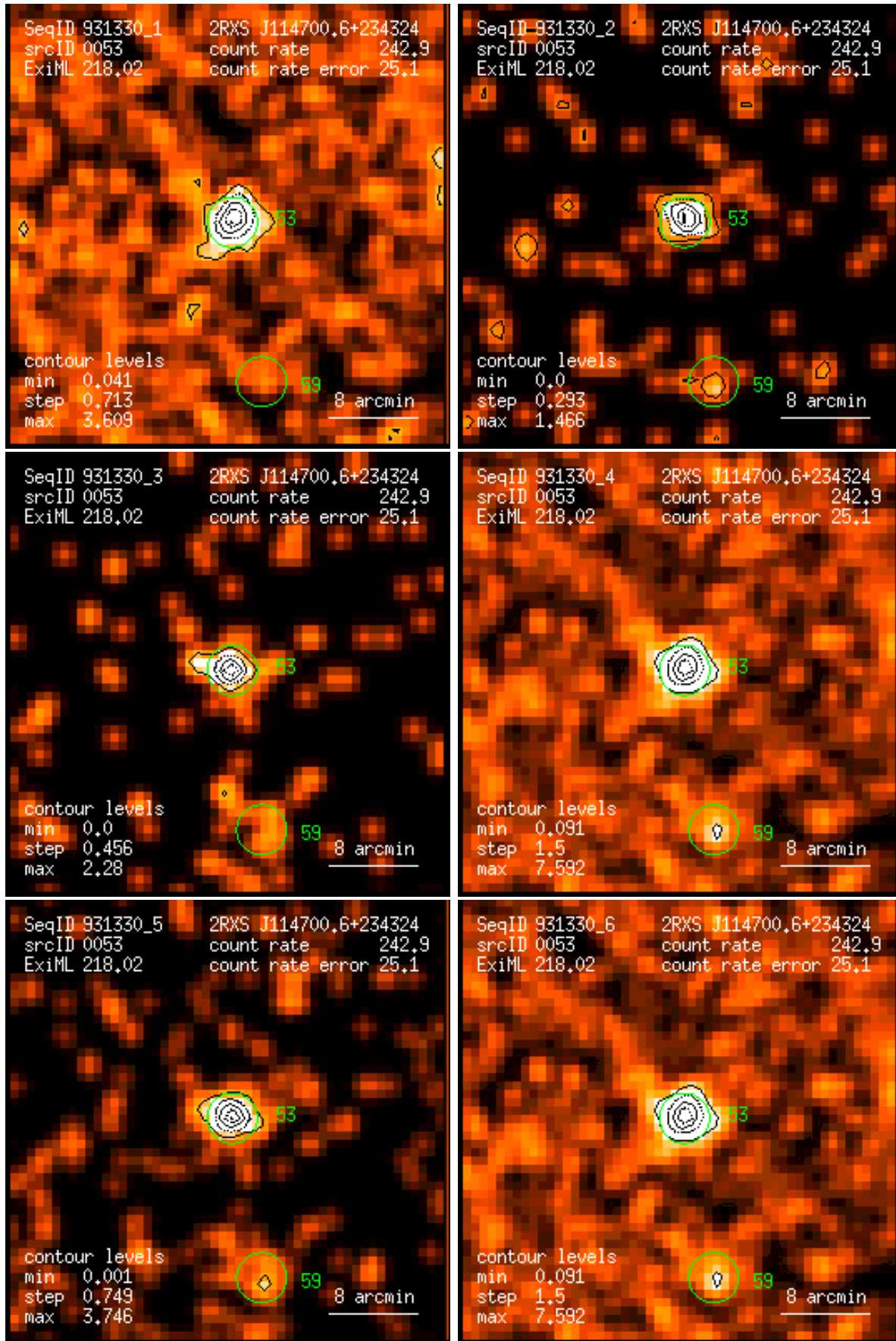
Figure 53: RASS 931330: detection 0053: band rate images, Gaussian filter: (1) PSPC channels 11 – 41, (2) 52 – 90, (3) 91 – 201, (4) 11 – 235, (5) 52 – 201, (6) 11 – 201. Broad band rates in counts/ks. Band rate contour levels in counts/ks/arcmin 2 .
