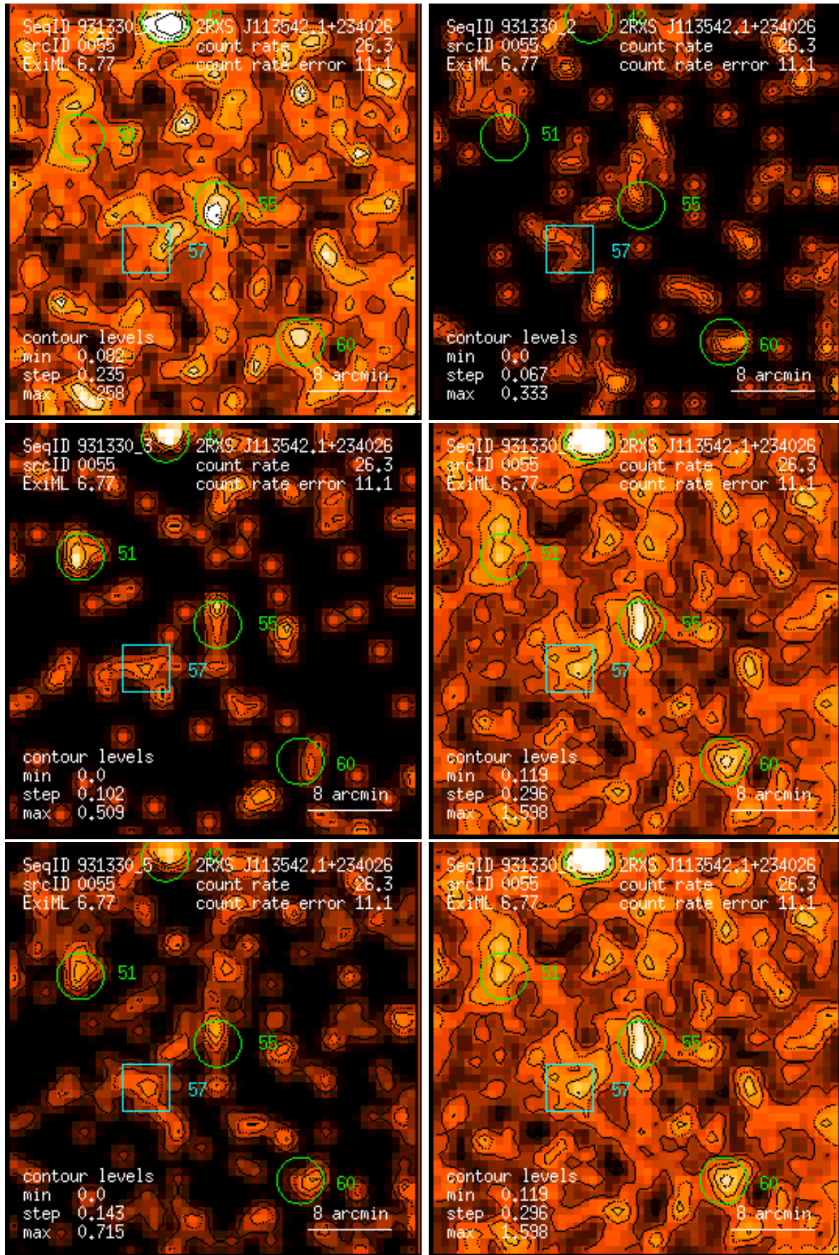
Figure 55: RASS 931330: detection 0055: band rate images, Gaussian filter: (1) PSPC channels 11 – 41, (2) 52 – 90, (3) 91 – 201, (4) 11 – 235, (5) 52 – 201, (6) 11 – 201. Broad band rates in counts/ks. Band rate contour levels in counts/ks/arcmin 2 .
