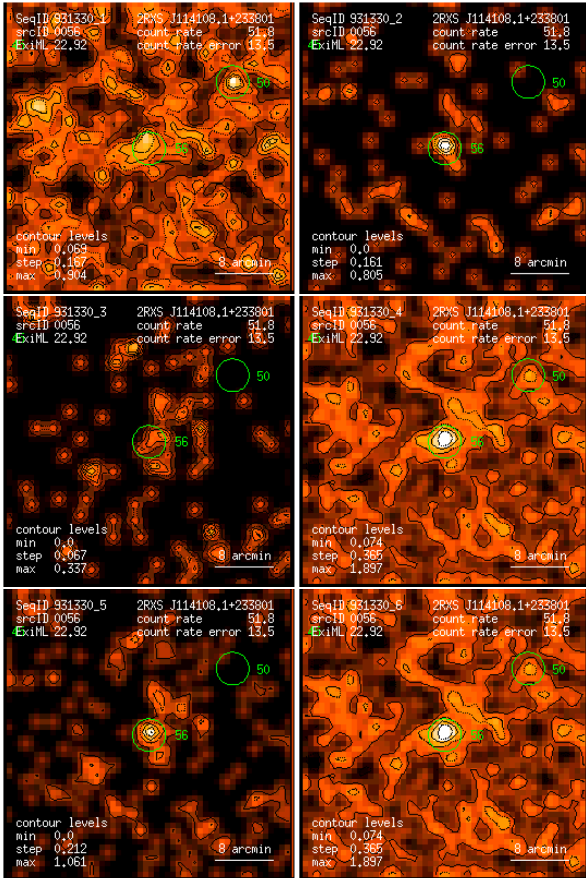
Figure 56: RASS 931330: detection 0056: band rate images, Gaussian filter: (1) PSPC channels 11 – 41, (2) 52 – 90, (3) 91 – 201, (4) 11 – 235, (5) 52 – 201, (6) 11 – 201. Broad band rates in counts/ks. Band rate contour levels in counts/ks/arcmin 2 .
