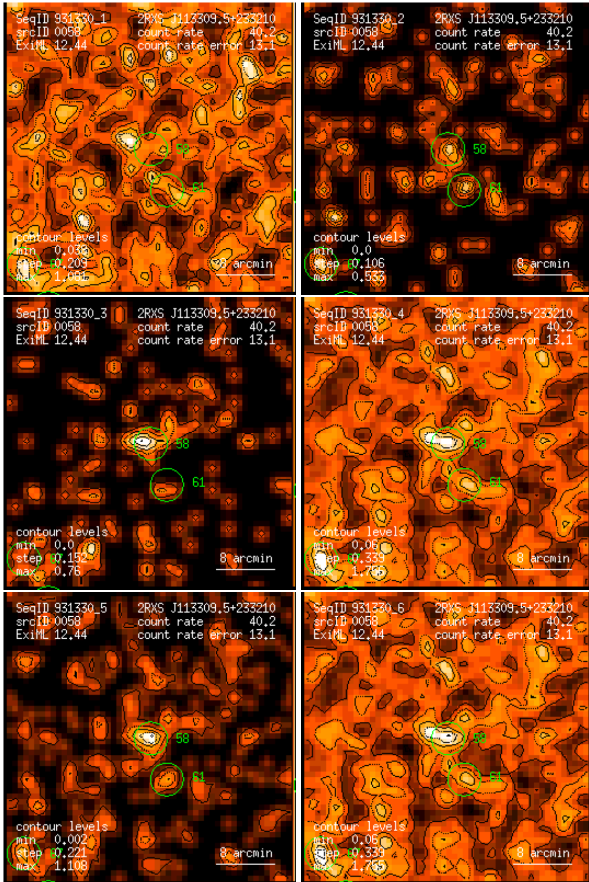
Figure 58: RASS 931330: detection 0058: band rate images, Gaussian filter: (1) PSPC channels 11 – 41, (2) 52 – 90, (3) 91 – 201, (4) 11 – 235, (5) 52 – 201, (6) 11 – 201. Broad band rates in counts/ks. Band rate contour levels in counts/ks/arcmin 2 .
