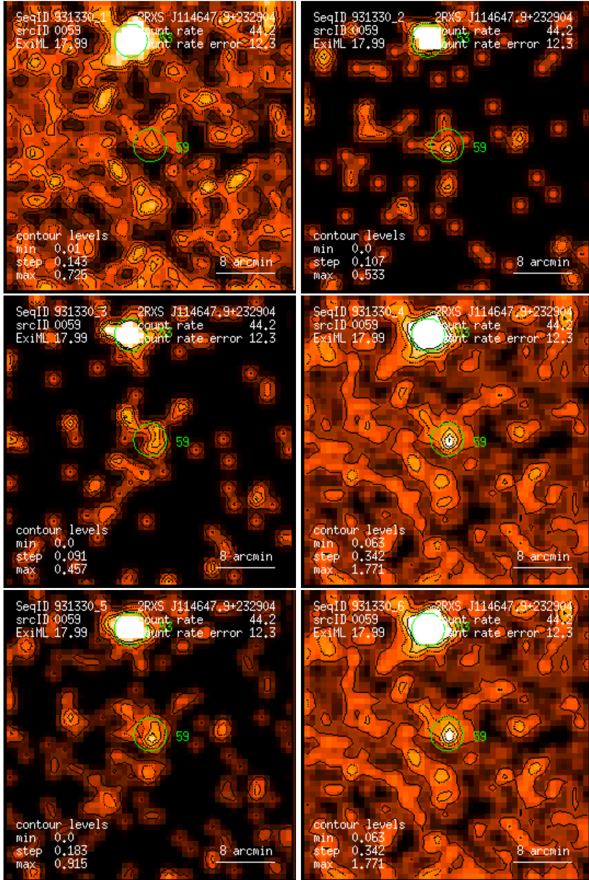
Figure 59: RASS 931330: detection 0059: band rate images, Gaussian filter: (1) PSPC channels 11 – 41, (2) 52 – 90, (3) 91 – 201, (4) 11 – 235, (5) 52 – 201, (6) 11 – 201. Broad band rates in counts/ks. Band rate contour levels in counts/ks/arcmin 2 .
