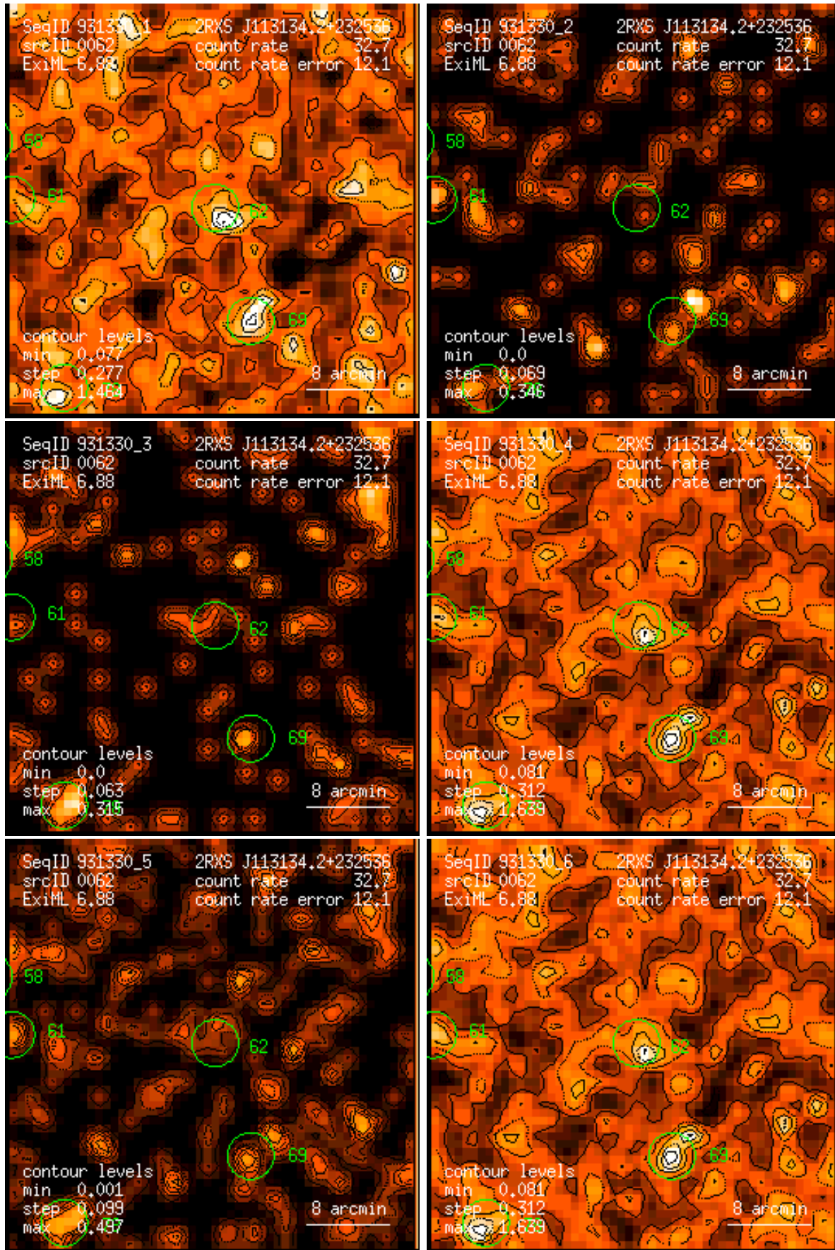
Figure 62: RASS 931330: detection 0062: band rate images, Gaussian filter: (1) PSPC channels 11 – 41, (2) 52 – 90, (3) 91 – 201, (4) 11 – 235, (5) 52 – 201, (6) 11 – 201. Broad band rates in counts/ks. Band rate contour levels in counts/ks/arcmin 2 .
