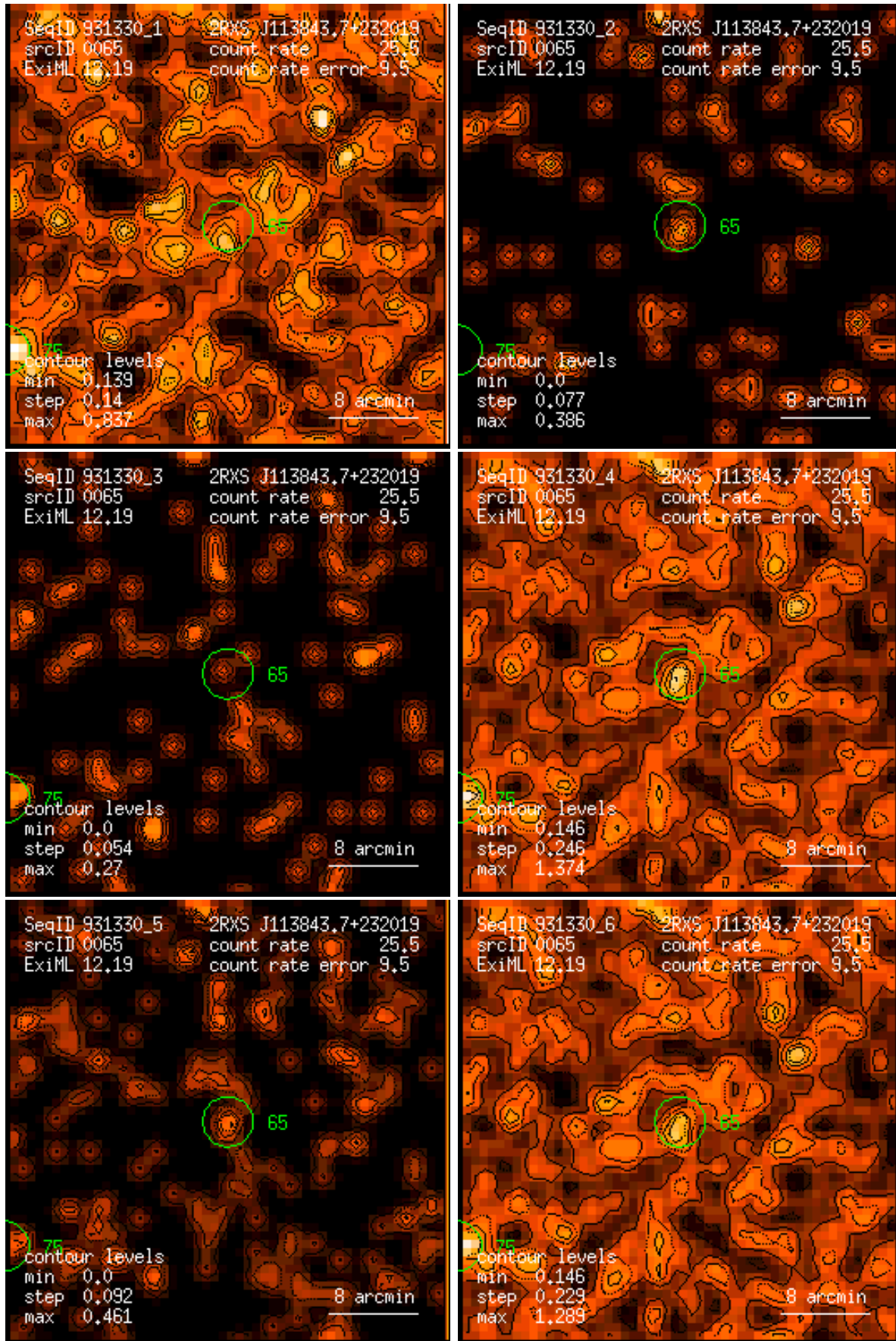
Figure 65: RASS 931330: detection 0065: band rate images, Gaussian filter: (1) PSPC channels 11 – 41, (2) 52 – 90, (3) 91 – 201, (4) 11 – 235, (5) 52 – 201, (6) 11 – 201. Broad band rates in counts/ks. Band rate contour levels in counts/ks/arcmin 2 .
