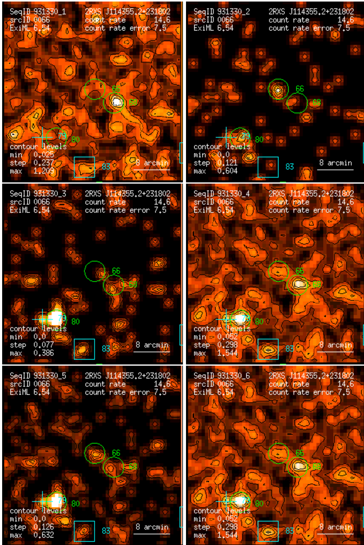
Figure 66: RASS 931330: detection 0066: band rate images, Gaussian filter: (1) PSPC channels 11 – 41, (2) 52 – 90, (3) 91 – 201, (4) 11 – 235, (5) 52 – 201, (6) 11 – 201. Broad band rates in counts/ks. Band rate contour levels in counts/ks/arcmin 2 .
