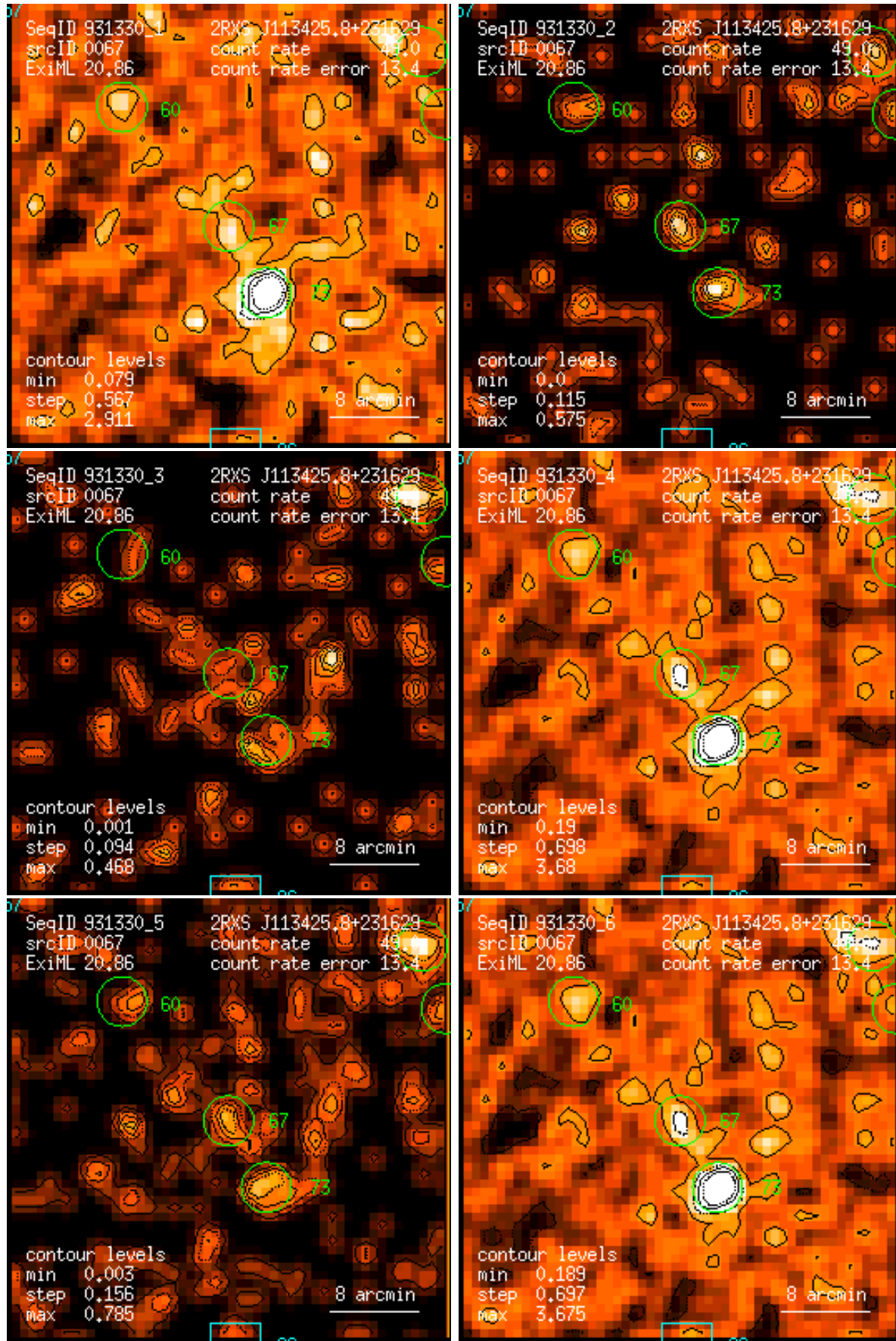
Figure 67: RASS 931330: detection 0067: band rate images, Gaussian filter: (1) PSPC channels 11 – 41, (2) 52 – 90, (3) 91 – 201, (4) 11 – 235, (5) 52 – 201, (6) 11 – 201. Broad band rates in counts/ks. Band rate contour levels in counts/ks/arcmin 2 .
