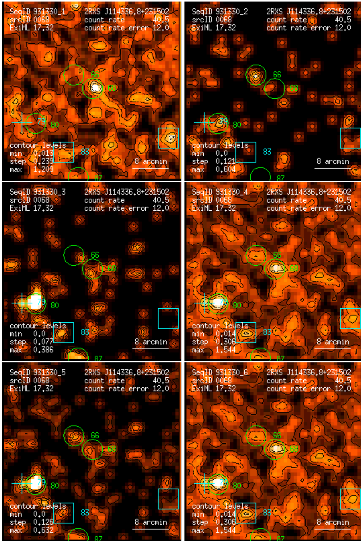
Figure 68: RASS 931330: detection 0068: band rate images, Gaussian filter: (1) PSPC channels 11 – 41, (2) 52 – 90, (3) 91 – 201, (4) 11 – 235, (5) 52 – 201, (6) 11 – 201. Broad band rates in counts/ks. Band rate contour levels in counts/ks/arcmin 2 .
