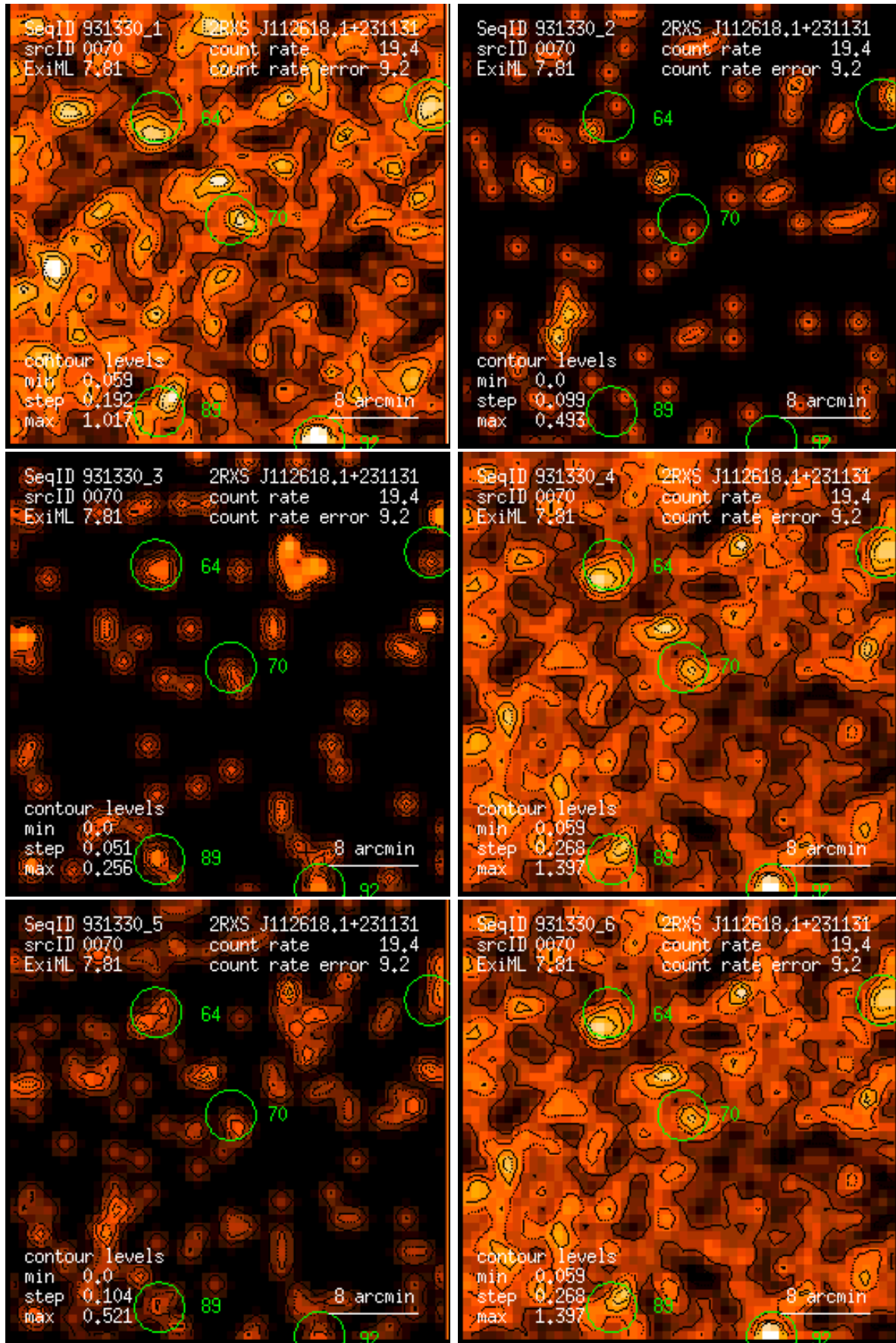
Figure 70: RASS 931330: detection 0070: band rate images, Gaussian filter: (1) PSPC channels 11 – 41, (2) 52 – 90, (3) 91 – 201, (4) 11 – 235, (5) 52 – 201, (6) 11 – 201. Broad band rates in counts/ks. Band rate contour levels in counts/ks/arcmin 2 .
