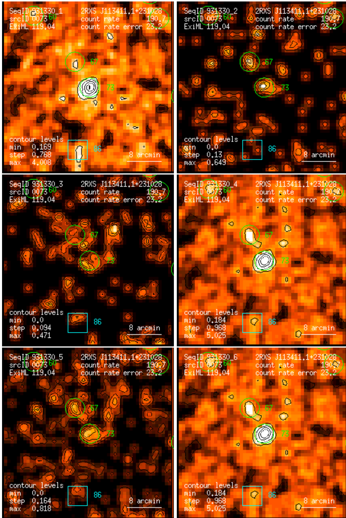
Figure 73: RASS 931330: detection 0073: band rate images, Gaussian filter: (1) PSPC channels 11 – 41, (2) 52 – 90, (3) 91 – 201, (4) 11 – 235, (5) 52 – 201, (6) 11 – 201. Broad band rates in counts/ks. Band rate contour levels in counts/ks/arcmin 2 .
