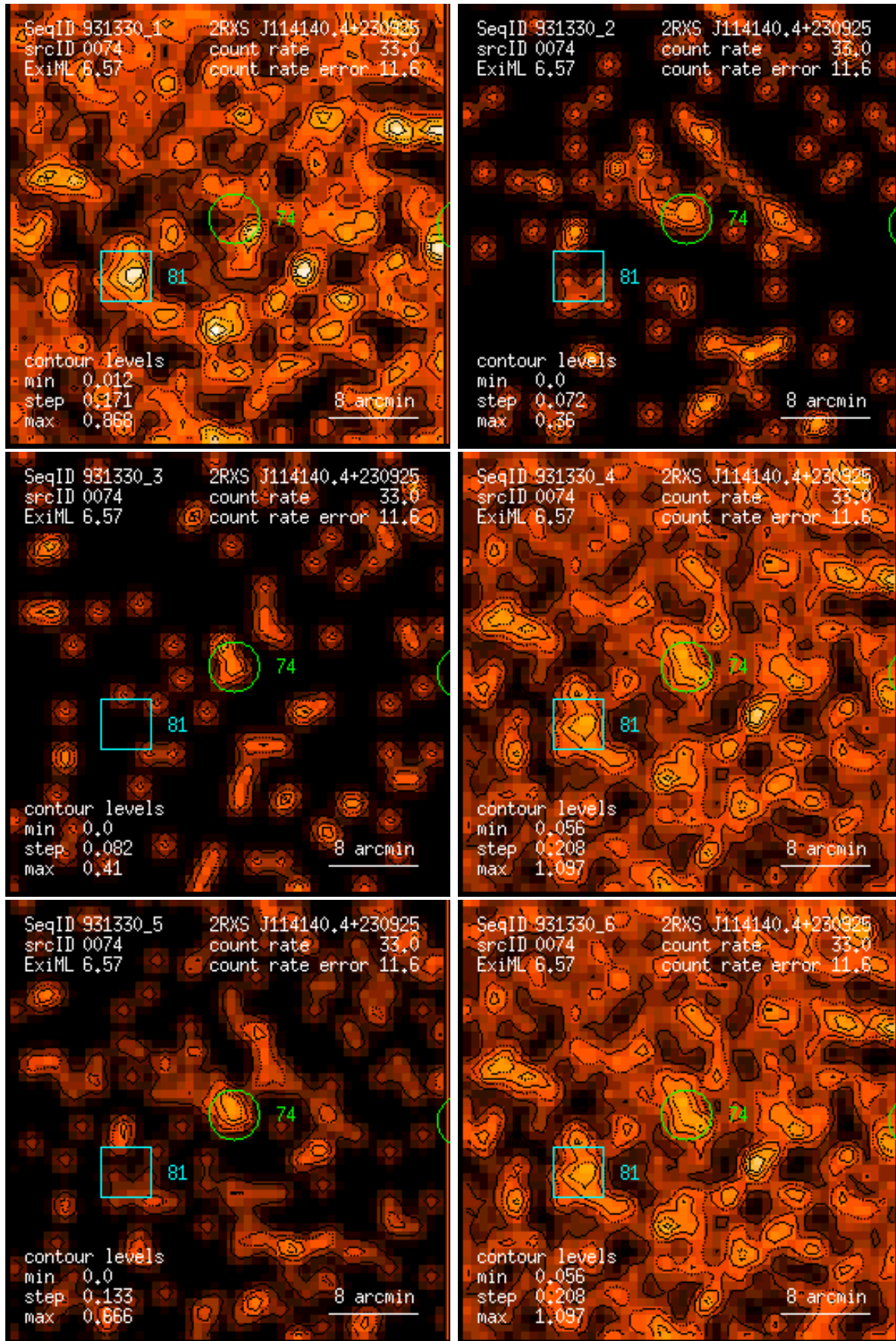
Figure 74: RASS 931330: detection 0074: band rate images, Gaussian filter: (1) PSPC channels 11 – 41, (2) 52 – 90, (3) 91 – 201, (4) 11 – 235, (5) 52 – 201, (6) 11 – 201. Broad band rates in counts/ks. Band rate contour levels in counts/ks/arcmin 2 .
