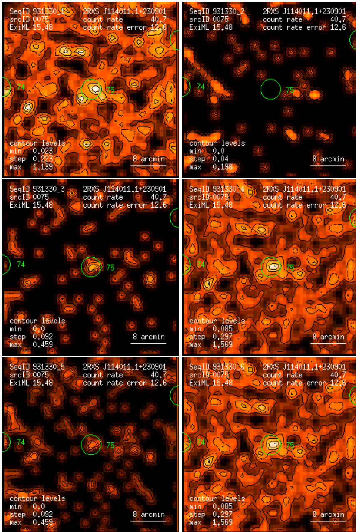
Figure 75: RASS 931330: detection 0075: band rate images, Gaussian filter: (1) PSPC channels 11 – 41, (2) 52 – 90, (3) 91 – 201, (4) 11 – 235, (5) 52 – 201, (6) 11 – 201. Broad band rates in counts/ks. Band rate contour levels in counts/ks/arcmin 2 .
