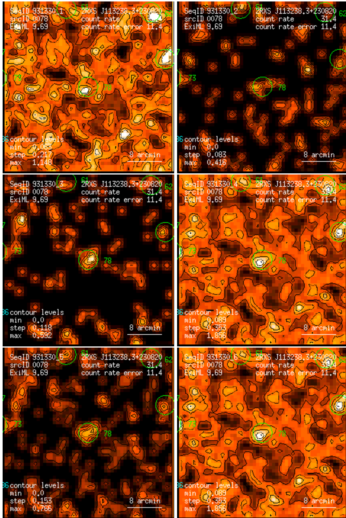
Figure 78: RASS 931330: detection 0078: band rate images, Gaussian filter: (1) PSPC channels 11 – 41, (2) 52 – 90, (3) 91 – 201, (4) 11 – 235, (5) 52 – 201, (6) 11 – 201. Broad band rates in counts/ks. Band rate contour levels in counts/ks/arcmin 2 .
