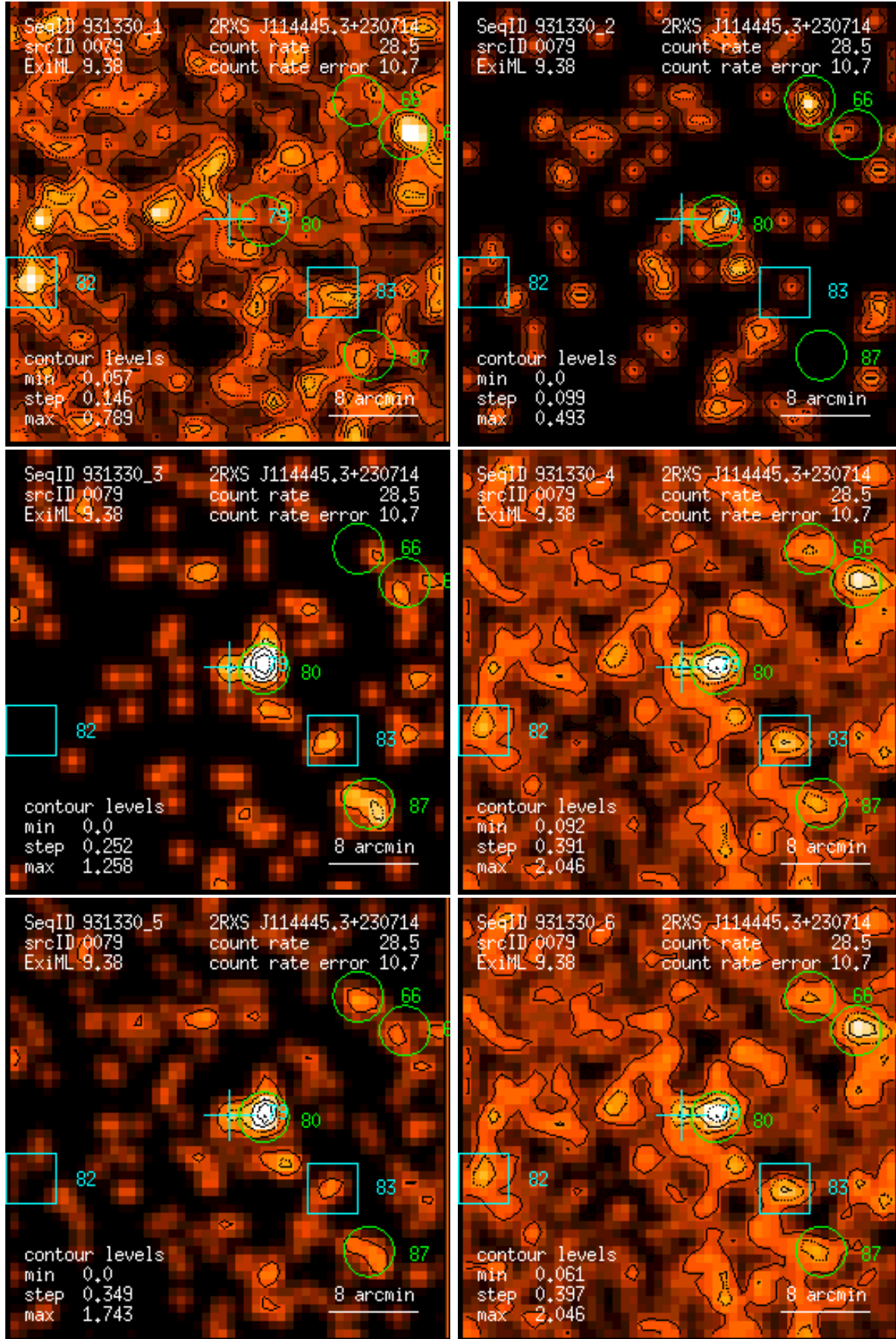
Figure 79: RASS 931330: detection 0079: band rate images, Gaussian filter: (1) PSPC channels 11 – 41, (2) 52 – 90, (3) 91 – 201, (4) 11 – 235, (5) 52 – 201, (6) 11 – 201. Broad band rates in counts/ks. Band rate contour levels in counts/ks/arcmin 2 .
