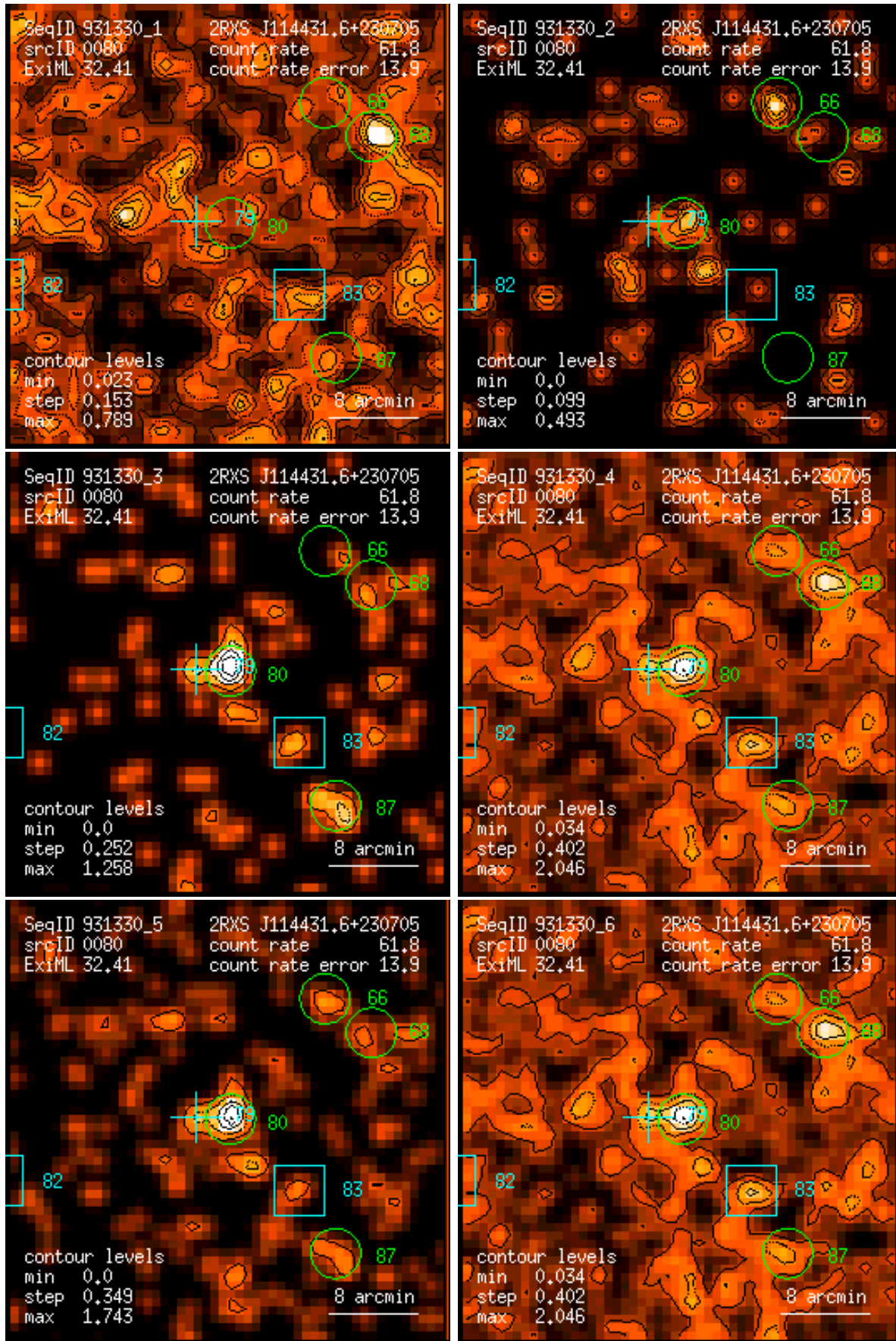
Figure 80: RASS 931330: detection 0080: band rate images, Gaussian filter: (1) PSPC channels 11 – 41, (2) 52 – 90, (3) 91 – 201, (4) 11 – 235, (5) 52 – 201, (6) 11 – 201. Broad band rates in counts/ks. Band rate contour levels in counts/ks/arcmin 2 .
