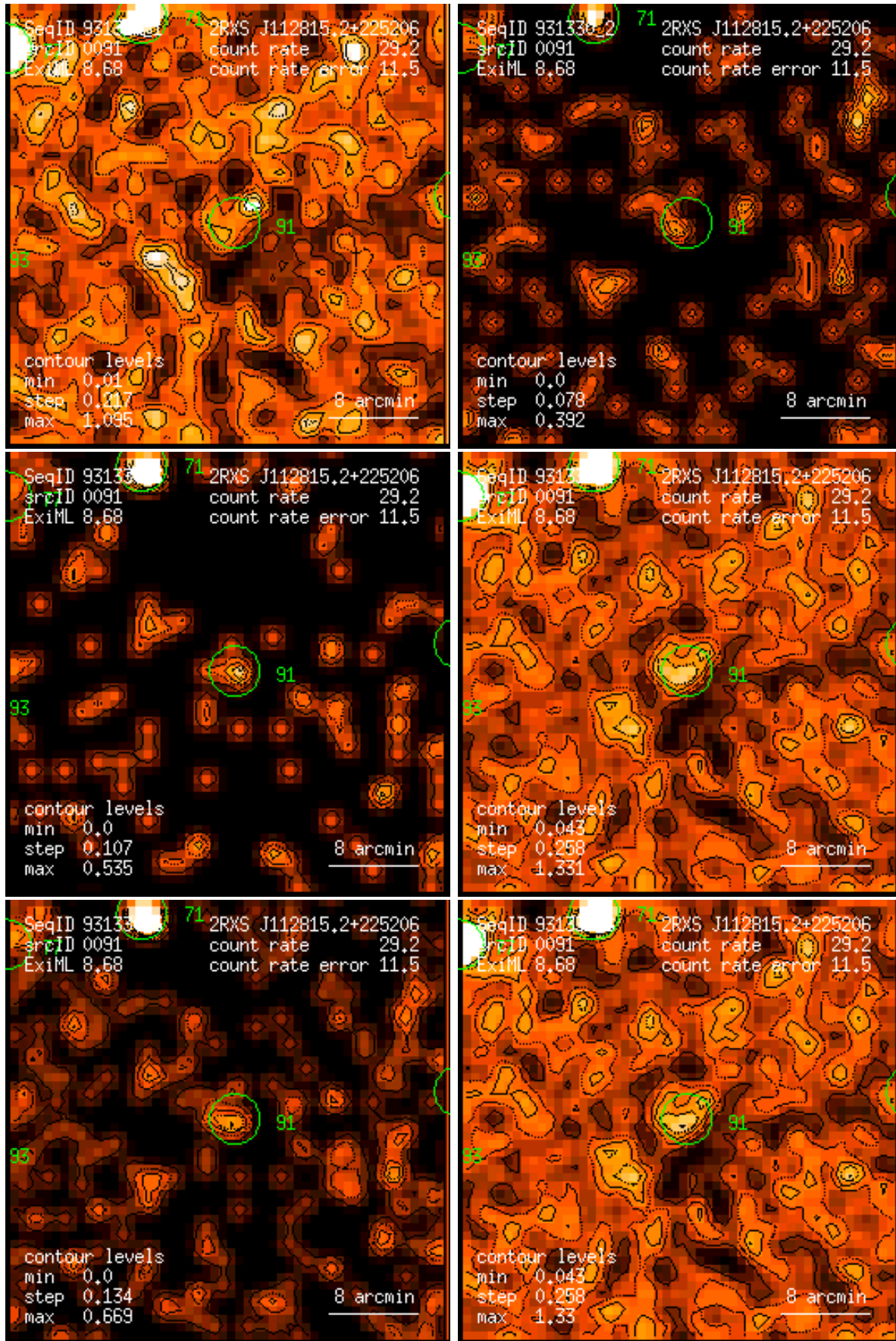
Figure 91: RASS 931330: detection 0091: band rate images, Gaussian filter: (1) PSPC channels 11 – 41, (2) 52 – 90, (3) 91 – 201, (4) 11 – 235, (5) 52 – 201, (6) 11 – 201. Broad band rates in counts/ks. Band rate contour levels in counts/ks/arcmin 2 .
