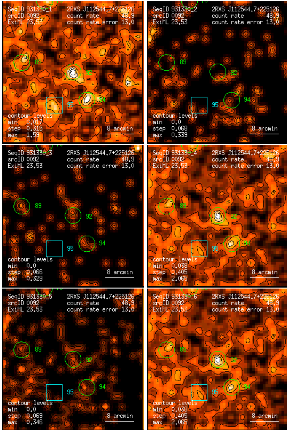
Figure 92: RASS 931330: detection 0092: band rate images, Gaussian filter: (1) PSPC channels 11 – 41, (2) 52 – 90, (3) 91 – 201, (4) 11 – 235, (5) 52 – 201, (6) 11 – 201. Broad band rates in counts/ks. Band rate contour levels in counts/ks/arcmin 2 .
