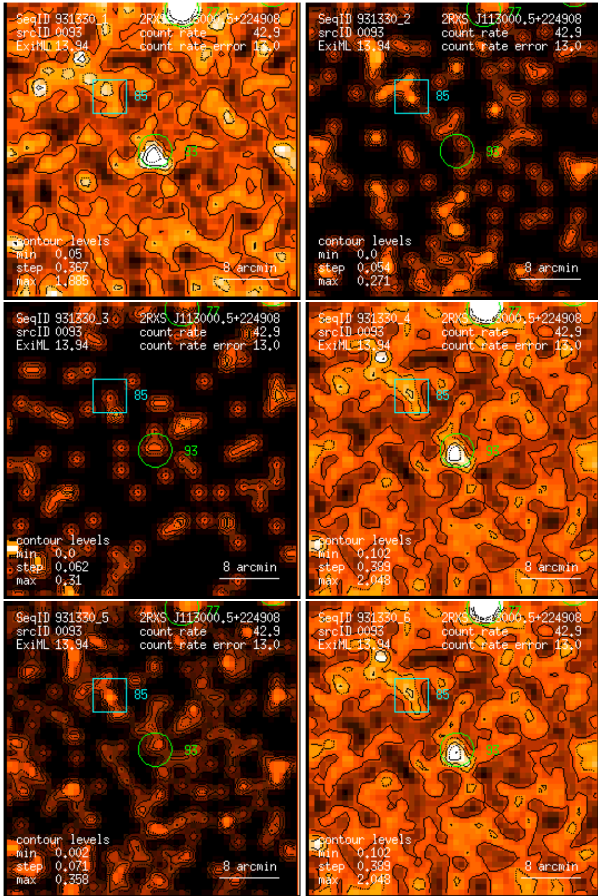
Figure 93: RASS 931330: detection 0093: band rate images, Gaussian filter: (1) PSPC channels 11 – 41, (2) 52 – 90, (3) 91 – 201, (4) 11 – 235, (5) 52 – 201, (6) 11 – 201. Broad band rates in counts/ks. Band rate contour levels in counts/ks/arcmin 2 .
