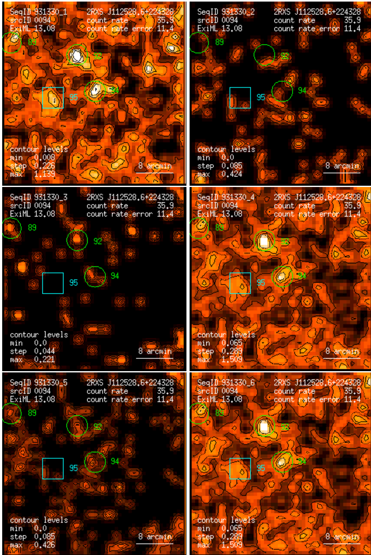
Figure 94: RASS 931330: detection 0094: band rate images, Gaussian filter: (1) PSPC channels 11 – 41, (2) 52 – 90, (3) 91 – 201, (4) 11 – 235, (5) 52 – 201, (6) 11 – 201. Broad band rates in counts/ks. Band rate contour levels in counts/ks/arcmin 2 .
