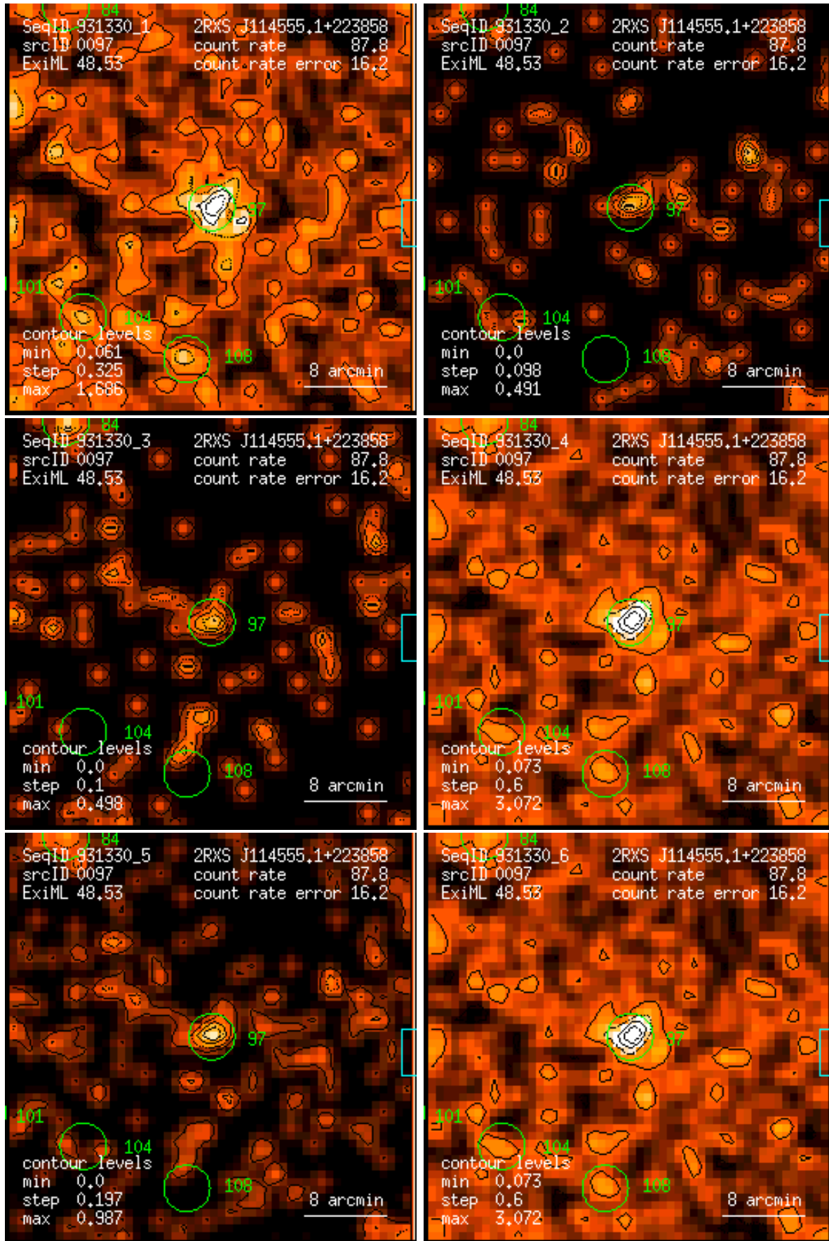
Figure 97: RASS 931330: detection 0097: band rate images, Gaussian filter: (1) PSPC channels 11 – 41, (2) 52 – 90, (3) 91 – 201, (4) 11 – 235, (5) 52 – 201, (6) 11 – 201. Broad band rates in counts/ks. Band rate contour levels in counts/ks/arcmin 2 .
