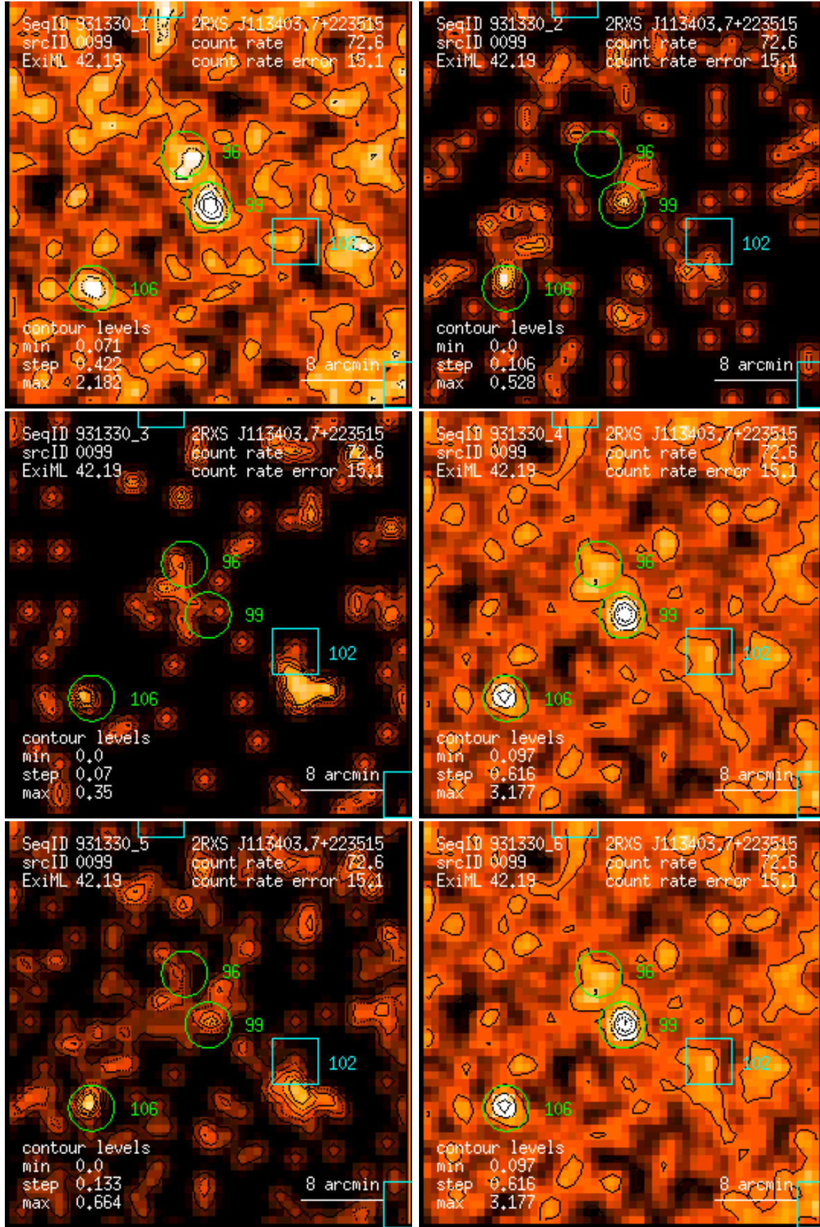
Figure 99: RASS 931330: detection 0099: band rate images, Gaussian filter: (1) PSPC channels 11 – 41, (2) 52 – 90, (3) 91 – 201, (4) 11 – 235, (5) 52 – 201, (6) 11 – 201. Broad band rates in counts/ks. Band rate contour levels in counts/ks/arcmin 2 .
